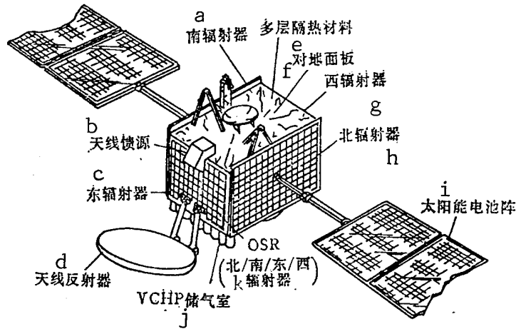
Fig. 5. Schematic diagram of thermal control scheme for communication satellite KEY: a - south radiator b - antenna feed source c - east radiator d - antenna reflector e - multilayer heat-insulating material f - ground-facing panel g - west radiator h - north radiator i - solar cell array j - gas storage chamber k - north/south/east/west radiators
