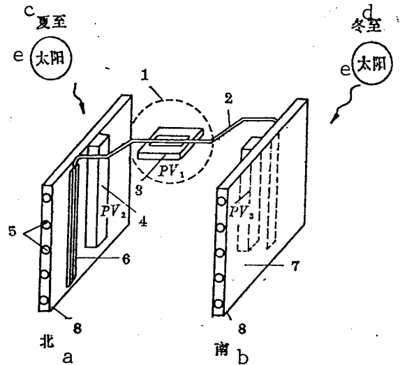
Fig. 3. Schematic diagram of south/north panels connected with heat pipe LEGEND: 1 - heat-insulating measure 2 - connecting heat pipe 3 - output multiplexer 4 - traveling-wave tube 5 - heat pipe buried within panel 6 - connecting heat pipe 7 - panel 8 - heat pipe radiator KEY: a - north b - south c - summer solstice d - winter solstice e - sun
