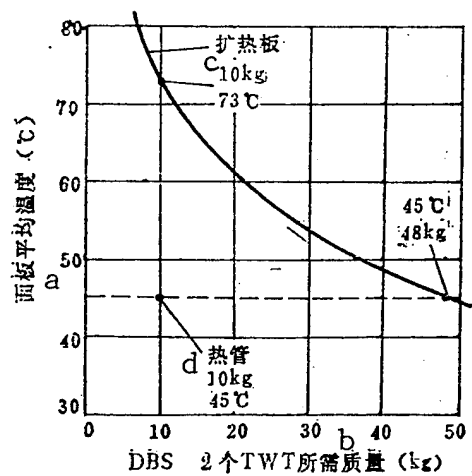
Fig. 2. Comparison between DBS heat pipe and expanded heating plate KEY: a - mean temperature of panel b - mass required for 2 TWT c - expanded heating plate d - heat pipe
