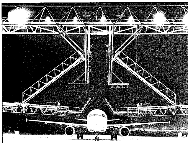
Centerpiece of the environmentally protective de-icing concept at the Munich Airport is the "Gantry", located to the east of the southern runway. This computer-controlled gantry can completely de-ice a B-747-400 in just under five minutes. Contaminated run-off water is drained into catch basins from which it is then fed into a recycling installation. (Photo Courtesy of Flughafen Munchen GmbH)
