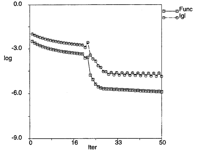
(b) SD2.
