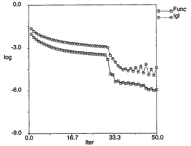
(c) SD2.
