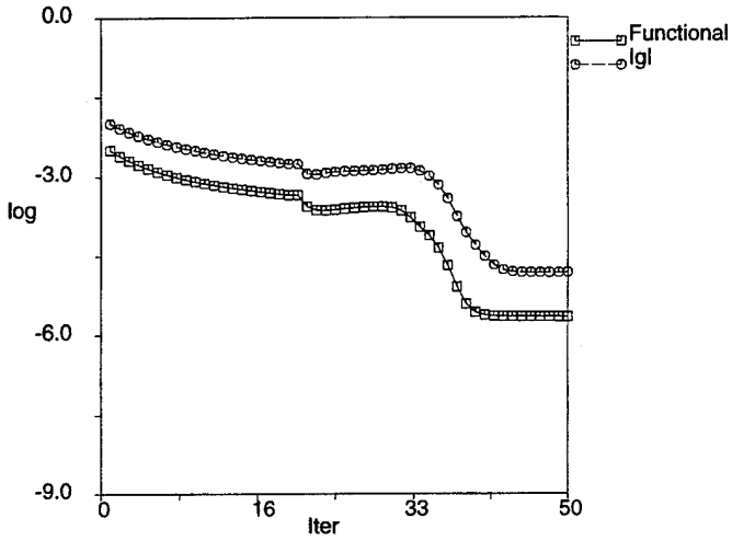
(c) BFGS1.
