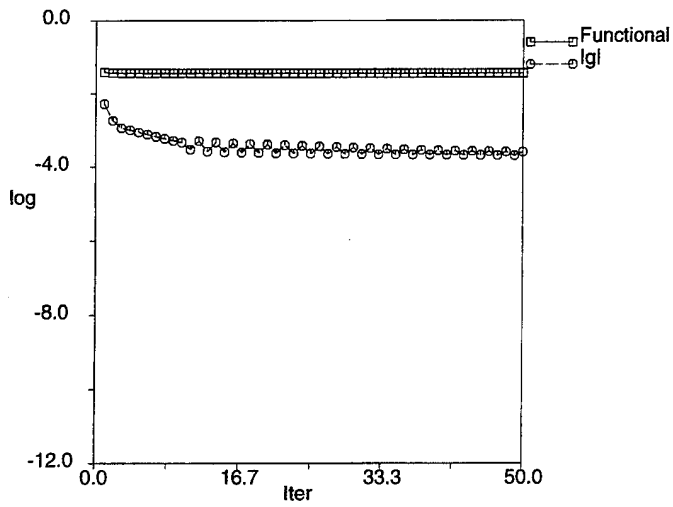
(a) DS2.
