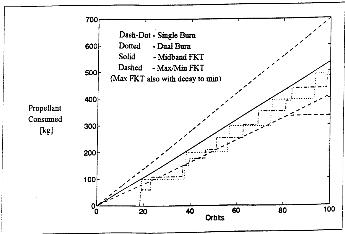
Figure 81. Propellant Consumption (25 km Bandwidth, 320 N Thrust)
