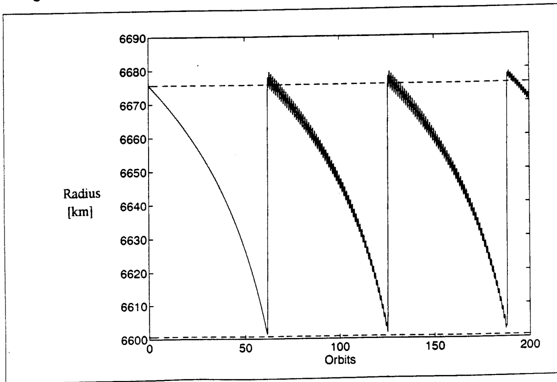
Figure 63. Dual Burn Strategy Orbital Radius (75 km Bandwidth, 320 N Thrust)
