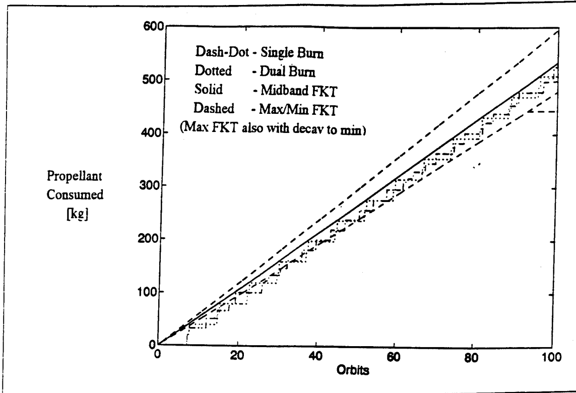
Figure 74. Propellant Consumption (10 km Bandwidth, 160 N Thrust)
