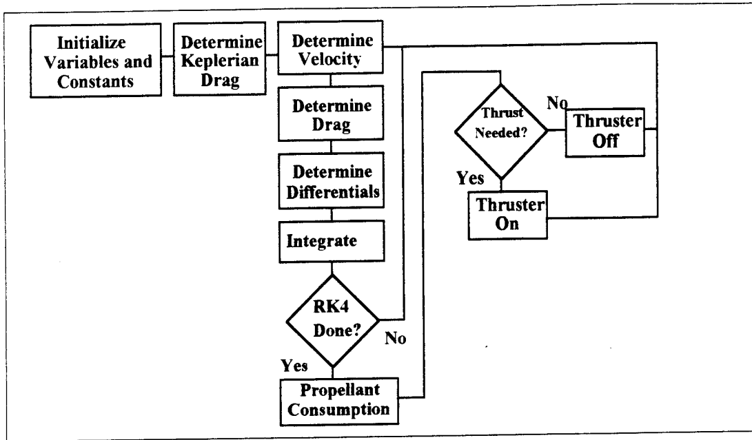
Figure 4. Program Flowchart
