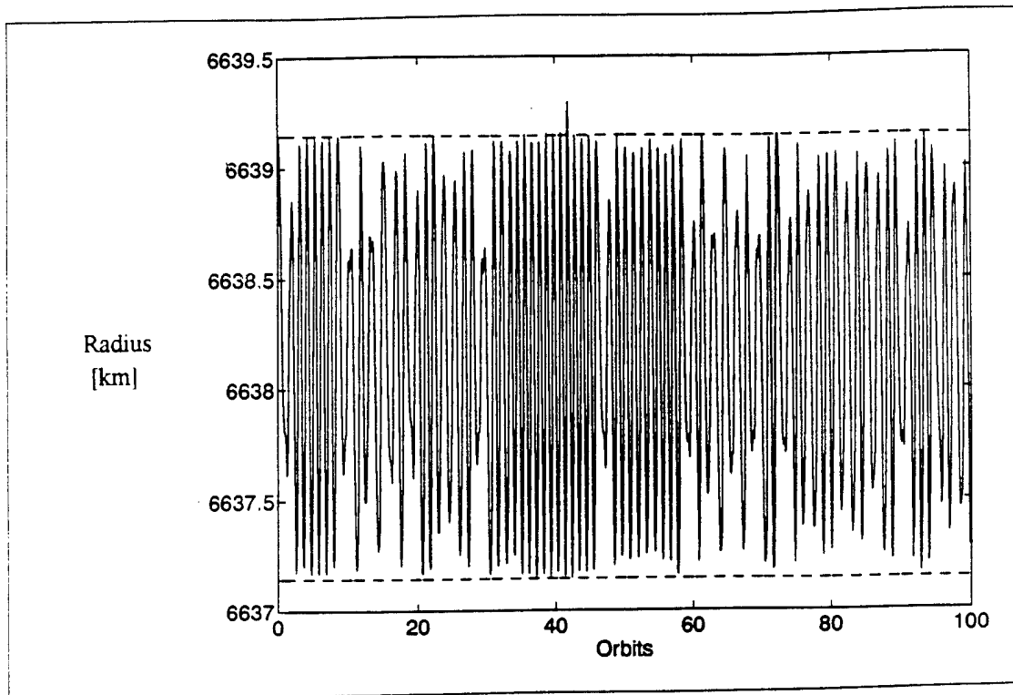
Figure 18. Single Burn Strategy Orbital Radius (2 km Bandwidth, 160 N Thrust)
