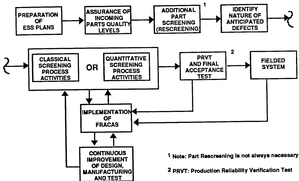
Figure 2.1. General ESS Process Flow Diagram
