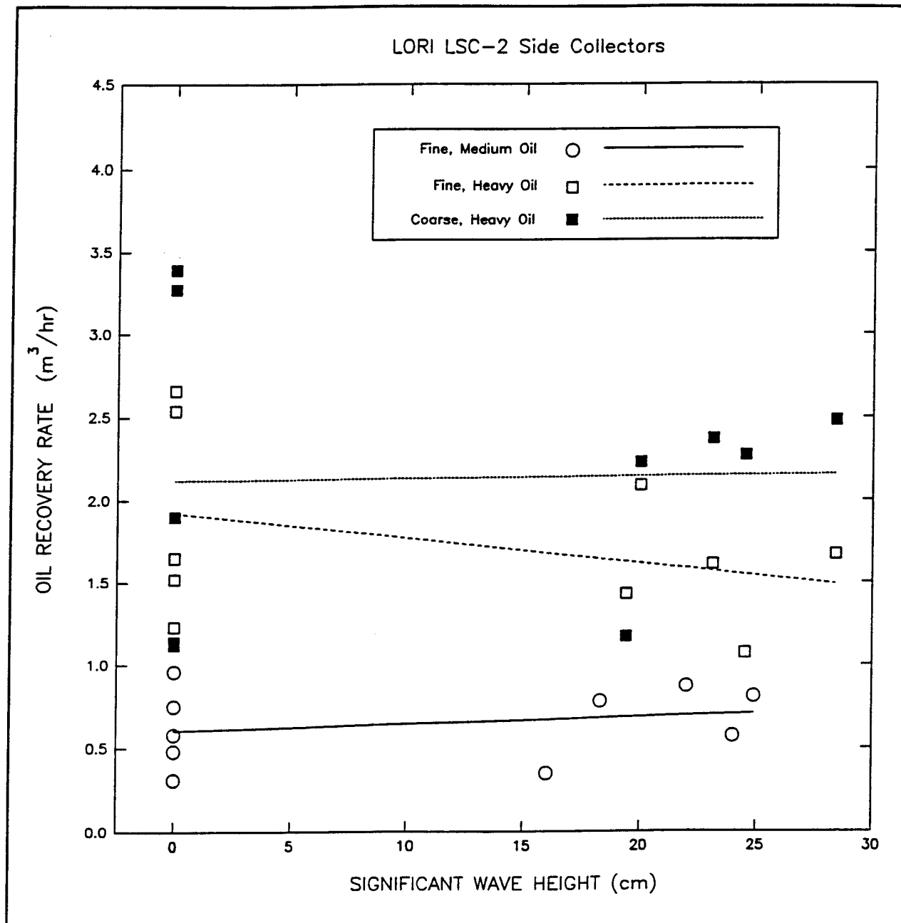
Figure 16. Oil Recovery Rate vs. Significant Wave Height, LORI, May 1993, at Ohmsett.
