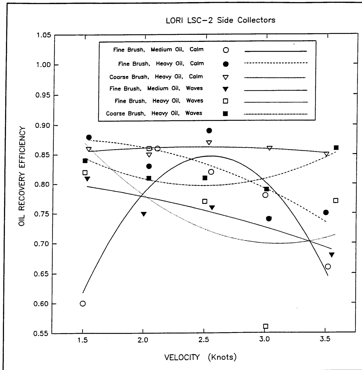
Figure 12. Oil Recovery Efficiency vs. Velocity, LORI, May 1993, at Ohmsett.
