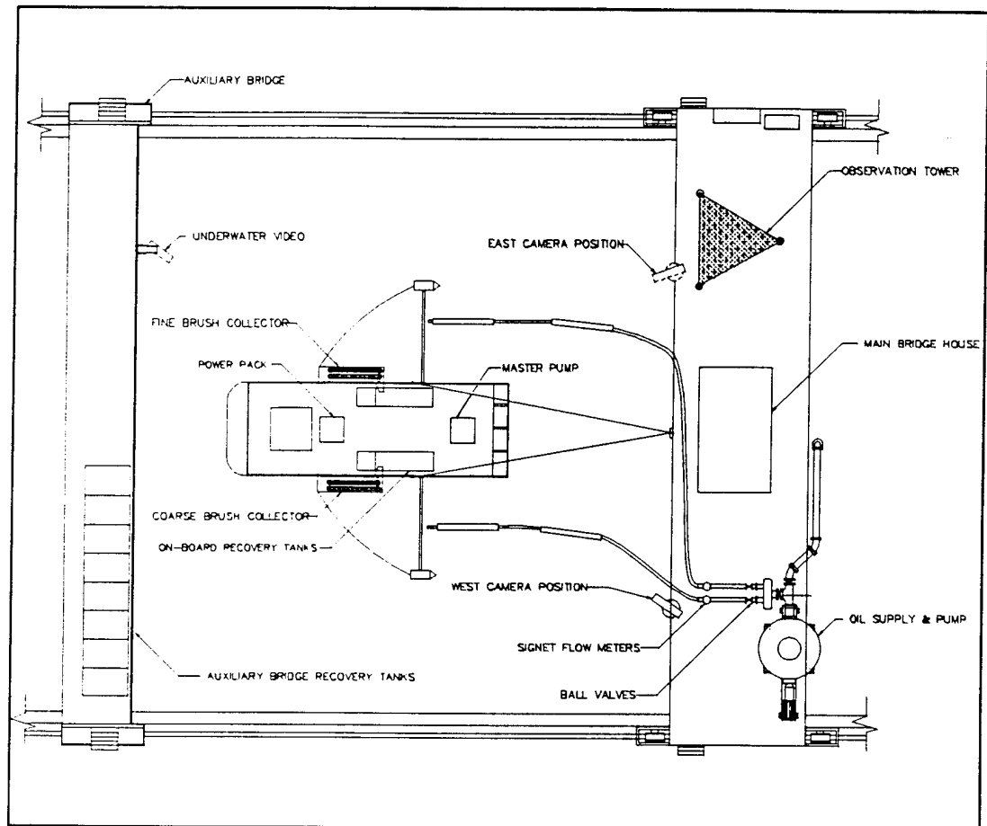
Figure 4. Test Configuration for LORI, May 1993, at Ohmsett.
