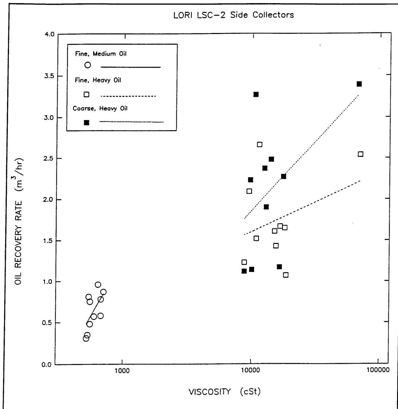
Figure 13. Oil Recovery Rate vs. Viscosity, LORI, May 1993, at Ohmsett.
