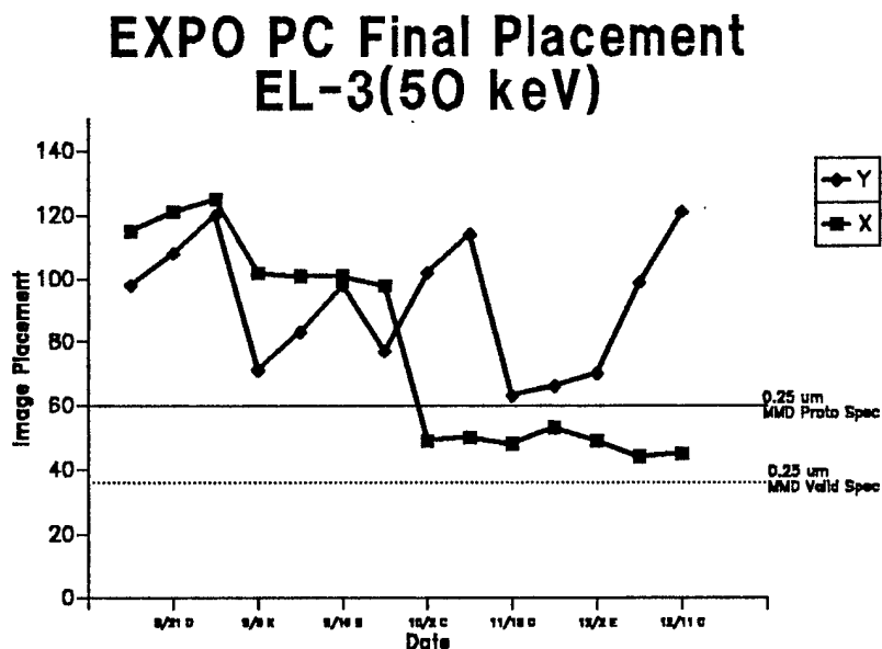
Figure 6. Final Placement Accuracy of EXPO PC Masks Written on EL-3+ (#6)
