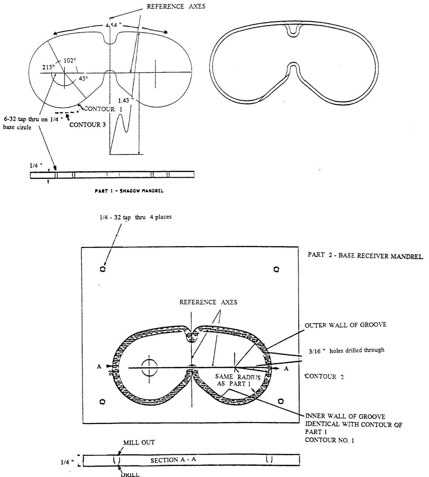
Figure 6. Holding fixture for thin film glass cutting, parts 1 and 2
