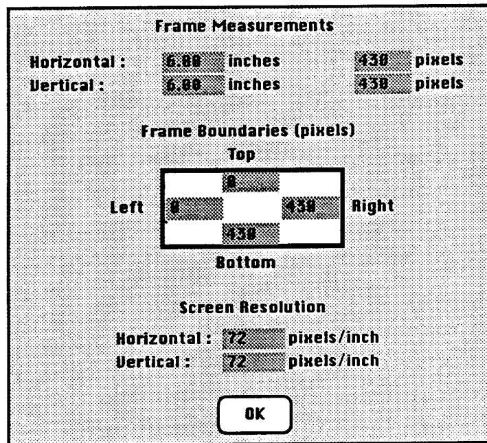
Figure 5-15. Graphics Window Summary Display
