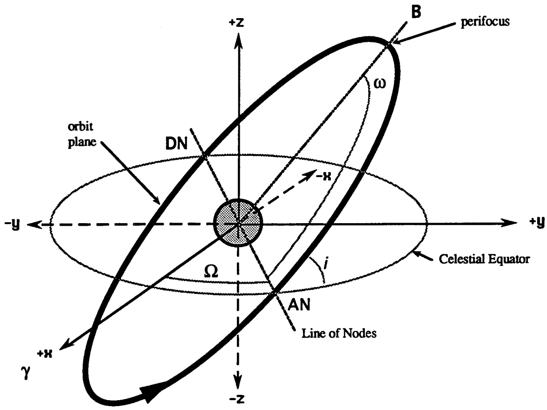
Figure C-3. Orientation of Orbit Ellipse Relative to Earth
