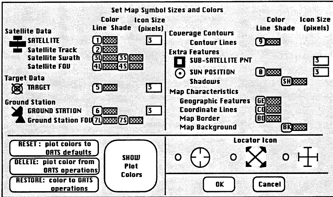
Figure 7-39. Master Dialog for Symbol Sizes and Colors
