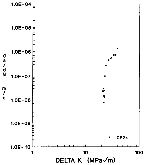
Fig. 13 PAF crack growth data, (a) a v N , (b) da/dN v \Delta K
