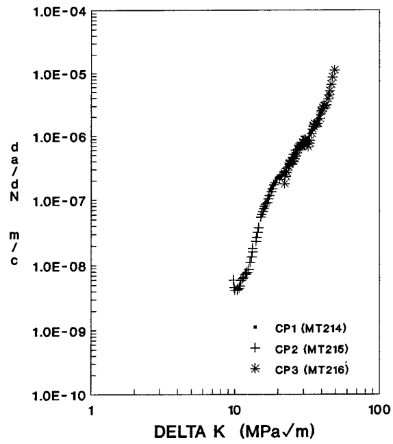
Fig. 10 GEC crack growth data, (a) a \text{ v } N , (b) da/dN \text{ v } \Delta K
