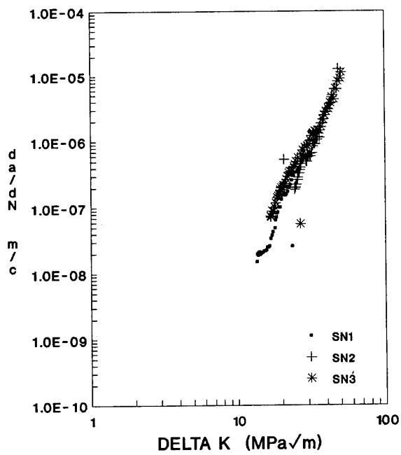
Fig. 11 SNECMA crack growth data, (a) a v N , (b) da/dN v \Delta K
