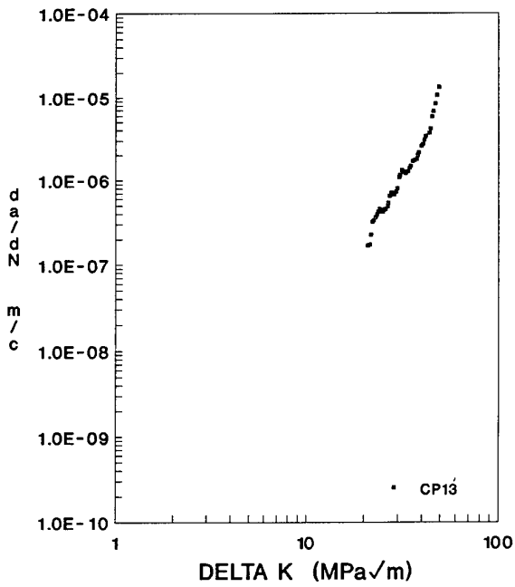
Fig. 9 KETA crack growth data, (a) a \text{ v } N , (b) da/dN \text{ v } \Delta K
