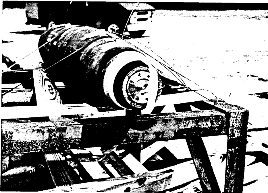
Figure 81: IMFT Fuzed Mk-82 Containing 4% Wax AFX-644 Fast Cook-Off Test Set Up
