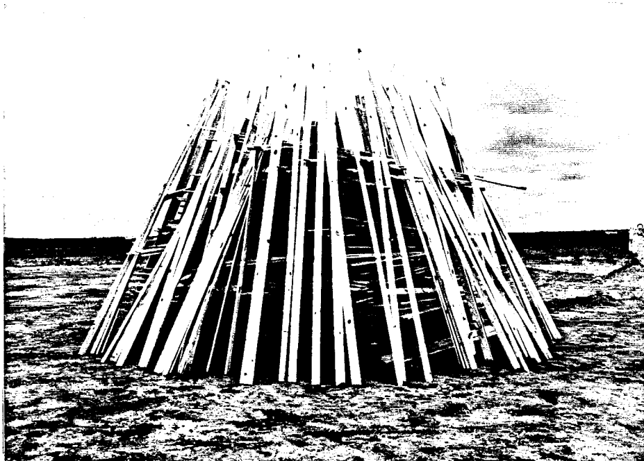
Figure 74: FIGPB Fast Cook-off Wood Bonfire Test
