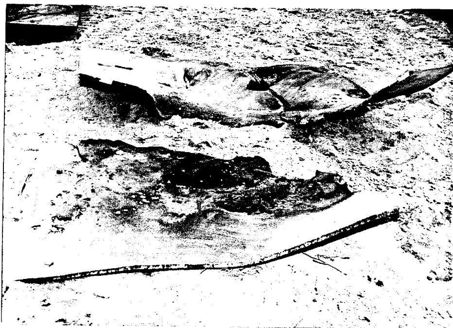
Figure 91: Top Witness Plate from All-up Round Sympathetic Detonation Test
