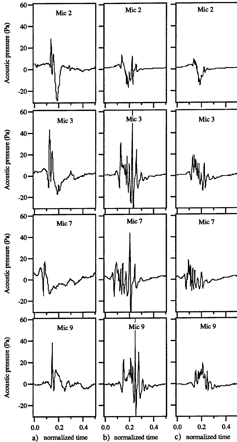
Fig. 13 Acoustic pressure is plotted as a function of normalized time (1 rev = 1 unit of time), column a) the measured acoustic pressure, column b) the acoustic pressure predicted using the compact formulation with FPR surface pressure with the wake shifted 0.25c, and column c) the acoustic pressure predicted using the compact formulation with FPR surface pressure with the wake shifted 0.50c.
