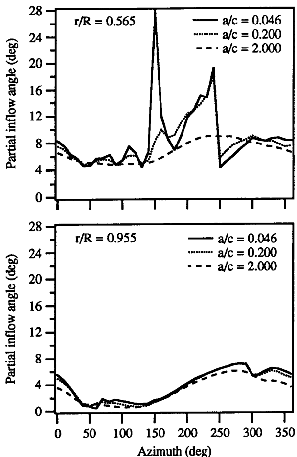
Fig. 1 CAMRAD/JA partial angles as a function of azimuth
