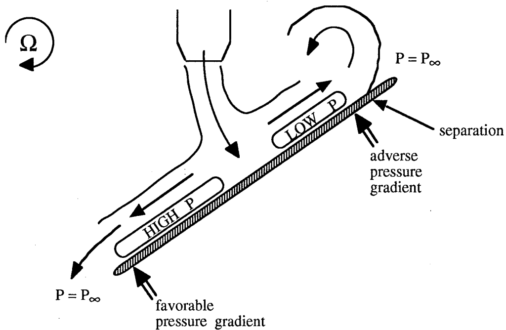
Figure 20. Effect of recovery to ambient pressure at plate edges
