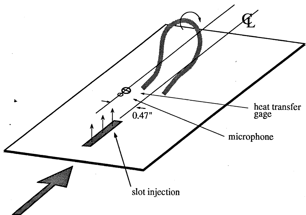
Figure 24. Heat transfer and pressure measurements: the gages are located outside the hairpin leg trajectory.
