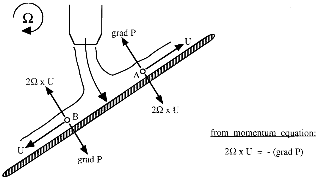
Figure 19. Lateral pressure gradients in wall jets
