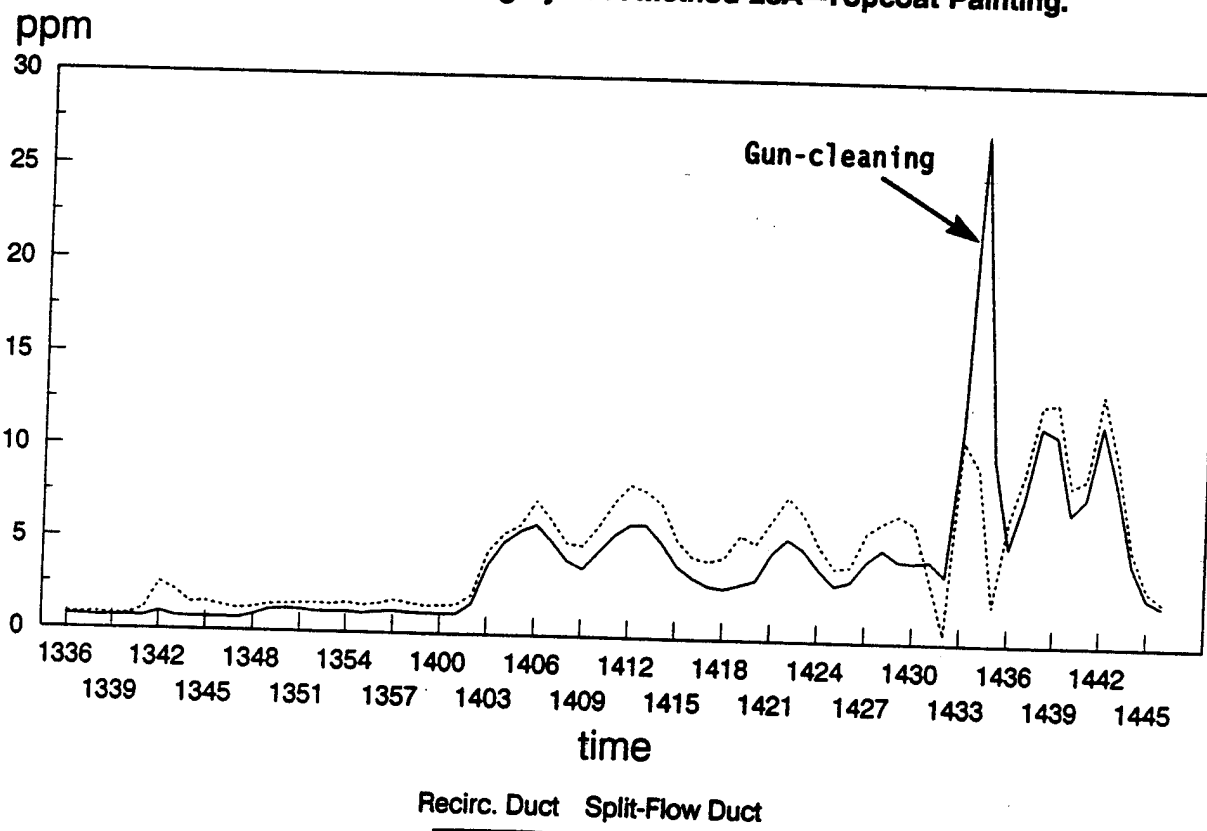
Figure 50. Representative Results from Continuous Emission Monitoring by EPA Method 25A—Primer Painting.
