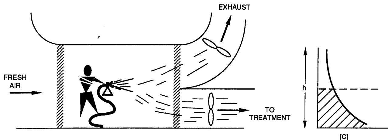
Figure 1. Schematic Diagram of a Split-Flow Ventilation System.
