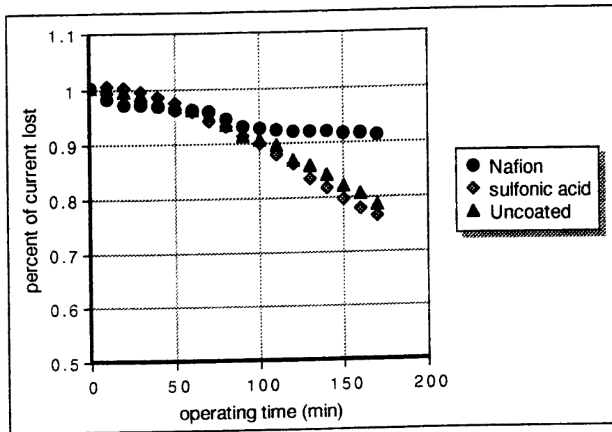
Fig. 8 Dependence of the steady-state current ratio over 170 min. operating time for an uncoated, chlorosulfonic acid treated, and a Nafion™ coated electrode: 1000 rpm, argon, 6 mM lactate.
