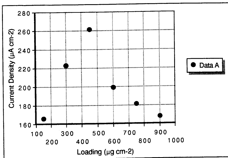
Fig. 5 Dependence of the limiting catalytic current density on the total amount of material coated on the electrode. Lactate sensors were prepared with a fixed wt. % of PVI 15 -Os-dmo-bpy (65%), LOx (26%), and PEGDGE (9%).
