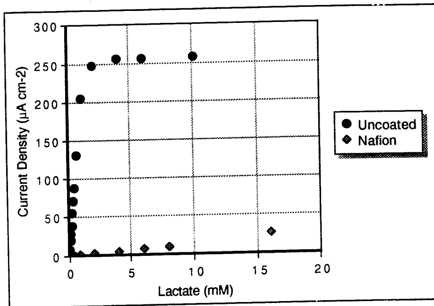
Fig. 9 Steady-state response of an uncoated and a Nafion™ coated electrode: 1000 rpm, argon.
