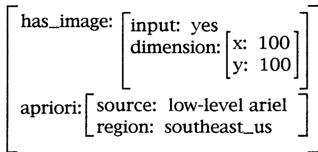
Figure 16. Feature Structure Subsumed by Figure 14 Feature Structures
