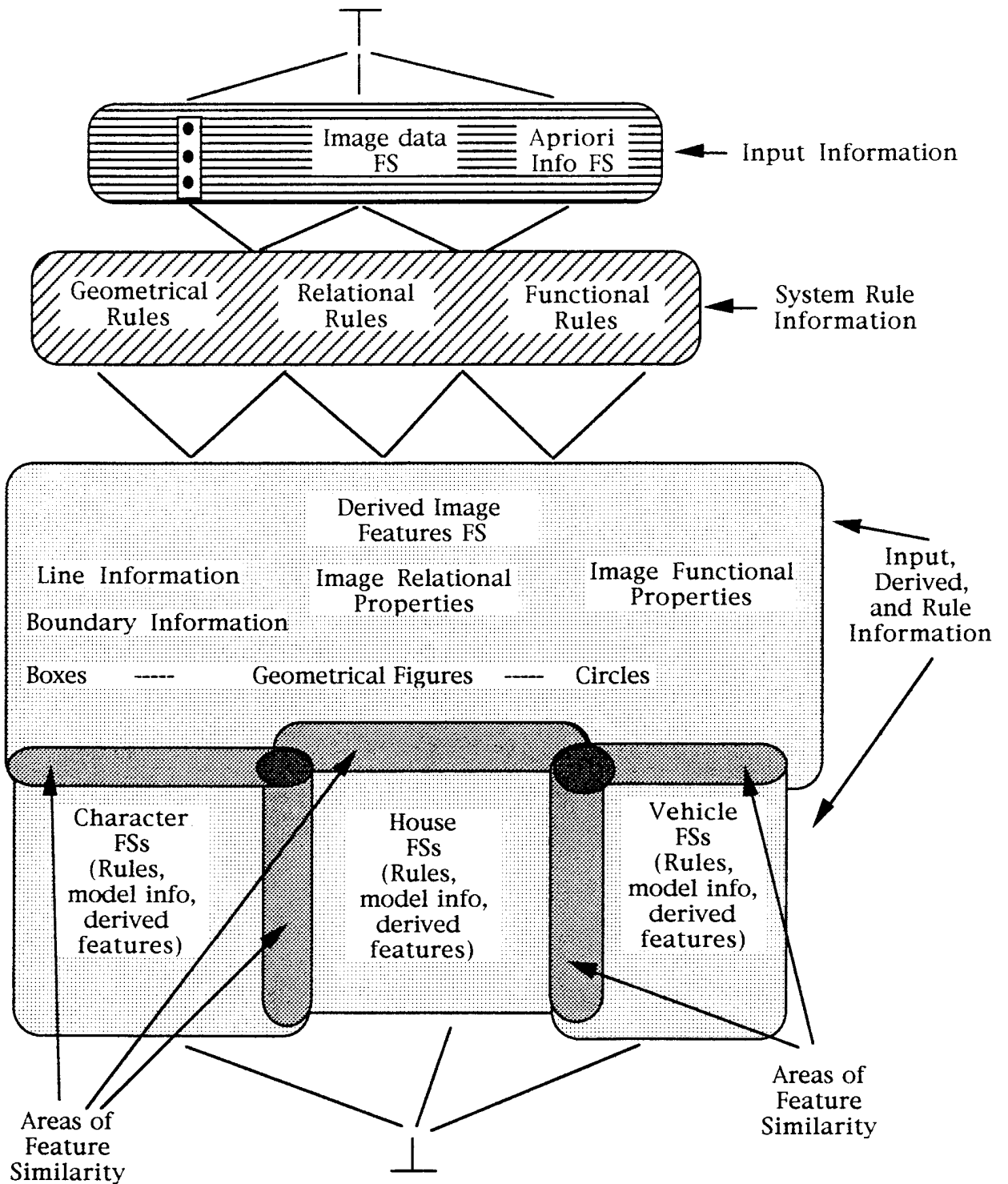
Figure 12. Locality of Information in a Lattice of Feature Structures
