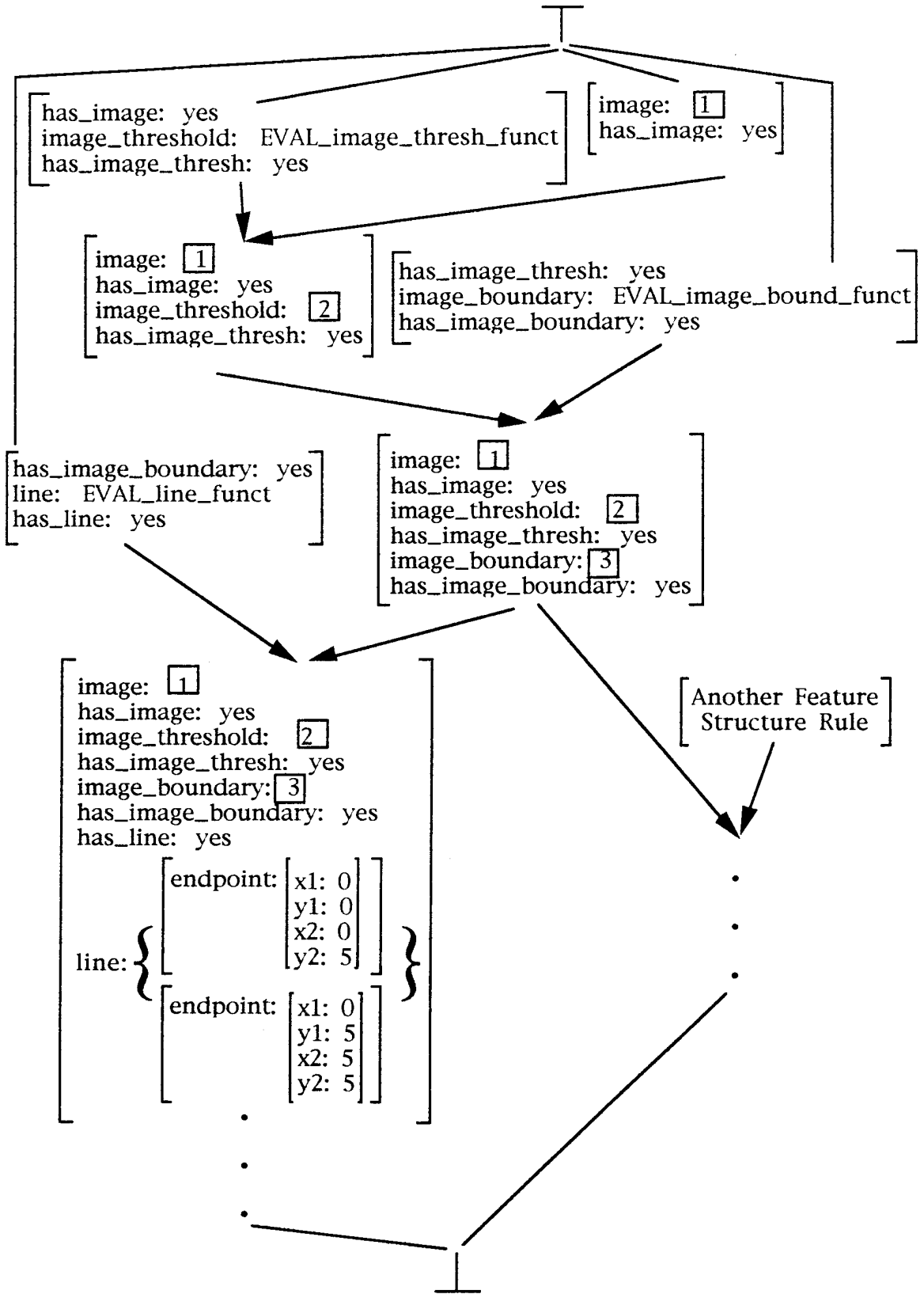
Figure 24. Initial Unifications of Input Feature Structures
