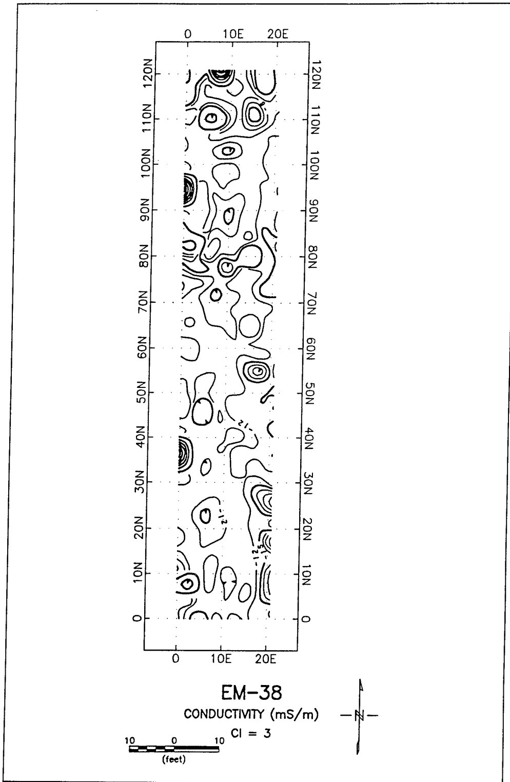
Figure 17. Contour map of conductivity data for east survey grid
