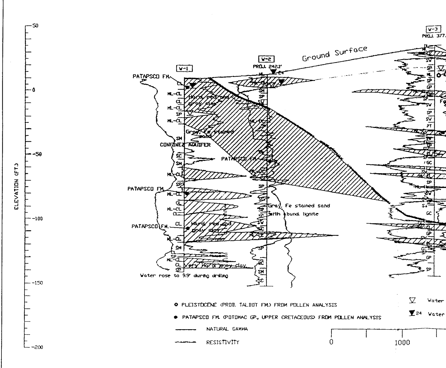
Figure 3. Stratigraphic cross section of Westwood Area
