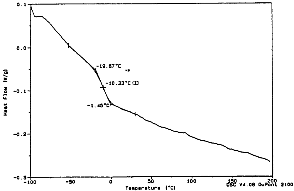
Figure 5. Differential scanning calorimeter (DSC) results for sample containing 38 percent by volume (3.00 percent by weight) microspheres.
