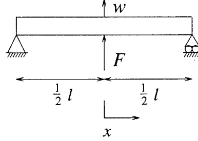
Figure 2.8: Pinned-Pinned Beam with Point Actuator-Sensor Pair
