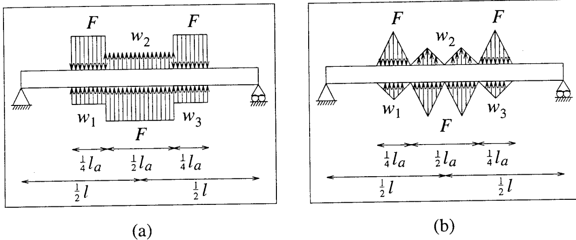
Figure 2.13: Pinned-Pinned Beams with Collocated Actuator-Sensor Pairs (a) Quadratic (b) Cubic
