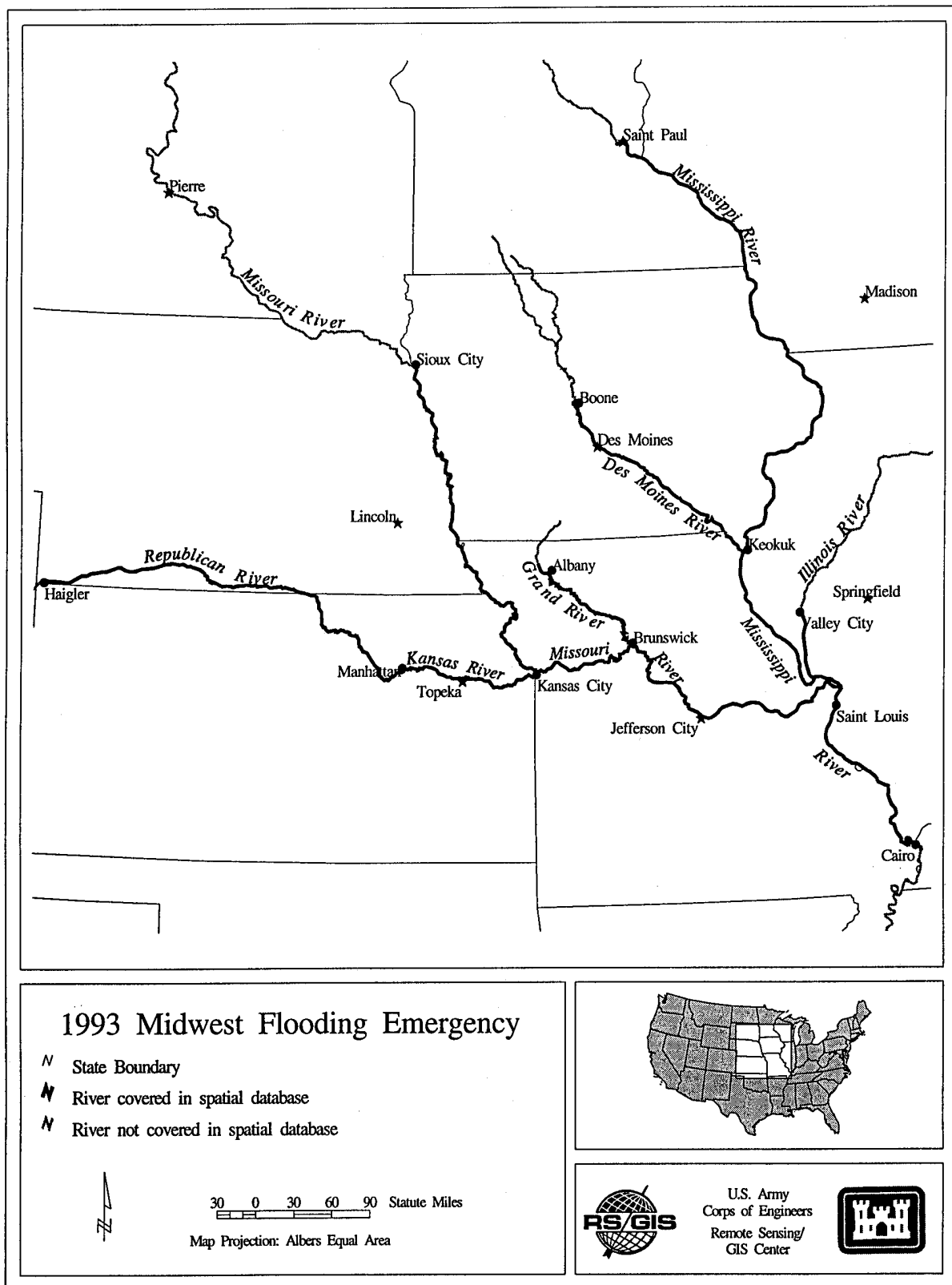
Figure 1. Seven rivers covered in the spatial database.
