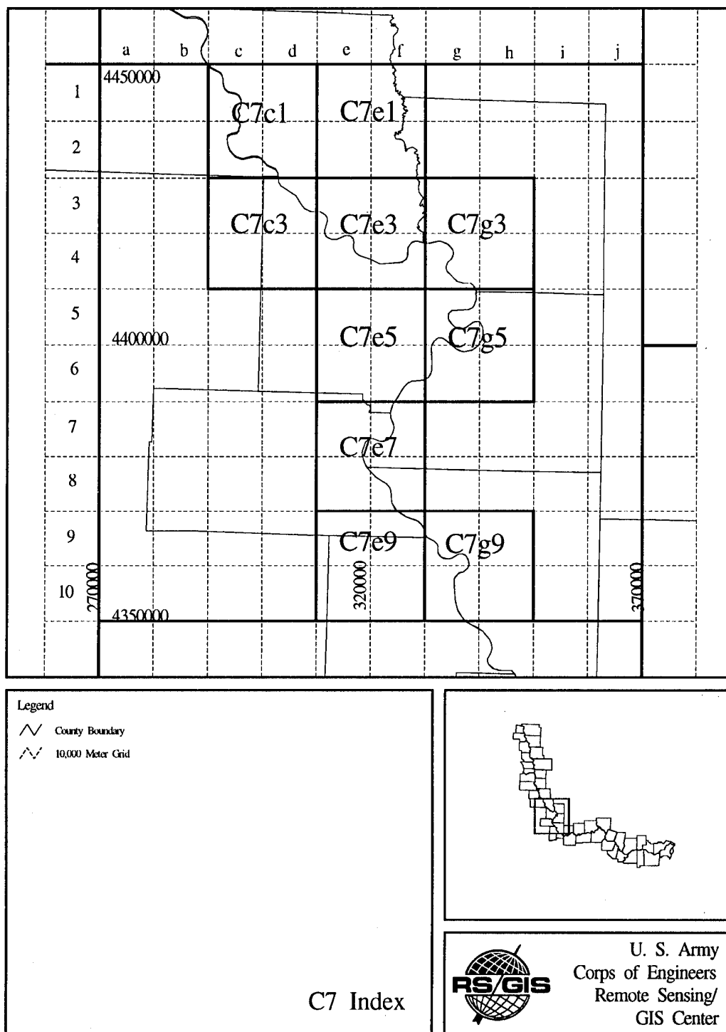
Figure 4. Index map for section C7, Missouri River, showing county boundaries, 10,000-m UTM grid and 20,000- x 20,000-m boxes. The projection is UTM zone 15.
