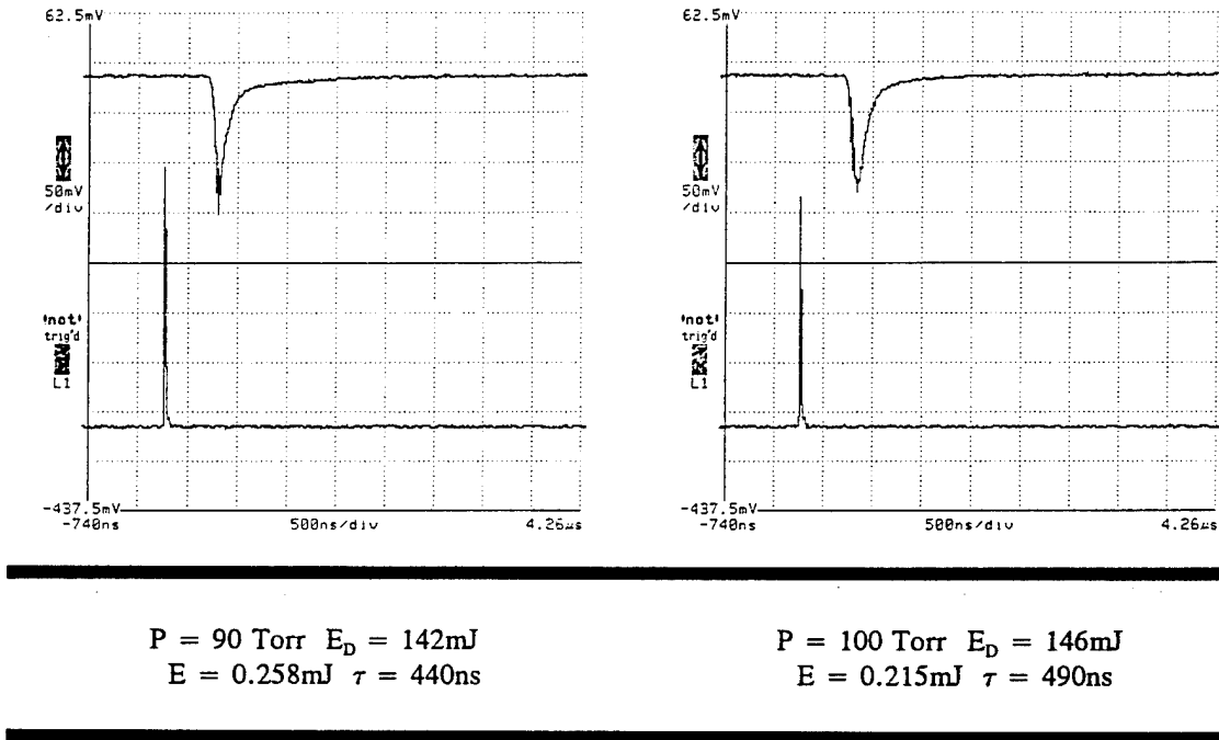
Figure 3-9 Varying \text{CF}_3\text{I} Pressure (continued)
