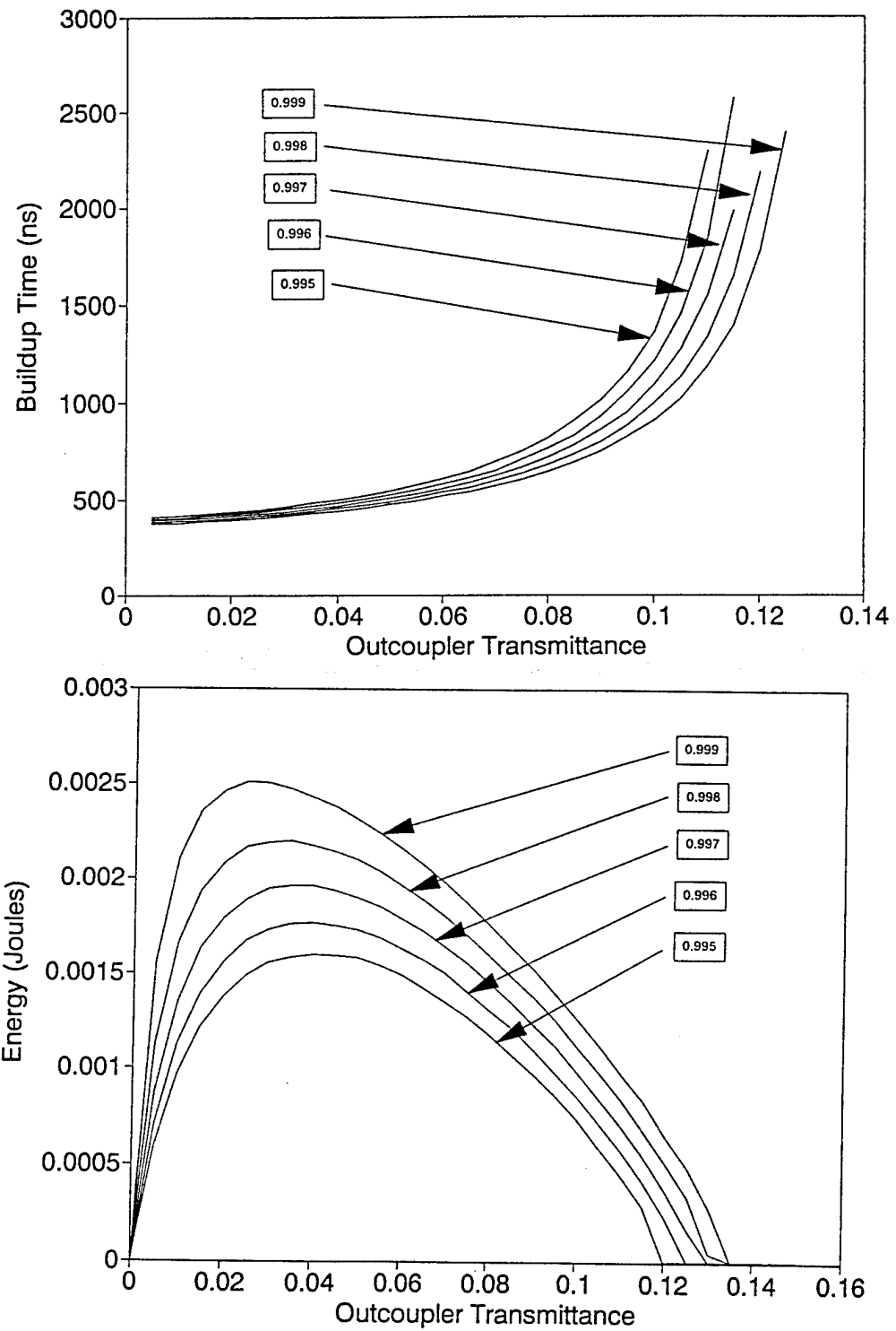
Figure 2-27 Result of Adding Window Transmission Loss
