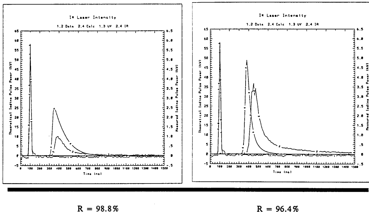
Figure 4-4 Qualitative Comparison of Laser Pulses for Various Outcoupling Mirrors
