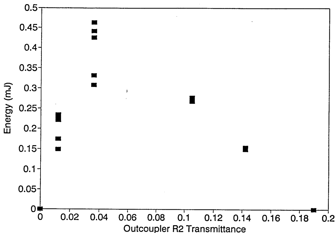
Figure 4-3 I^+ Laser Energy versus Outcoupler Transmittance
