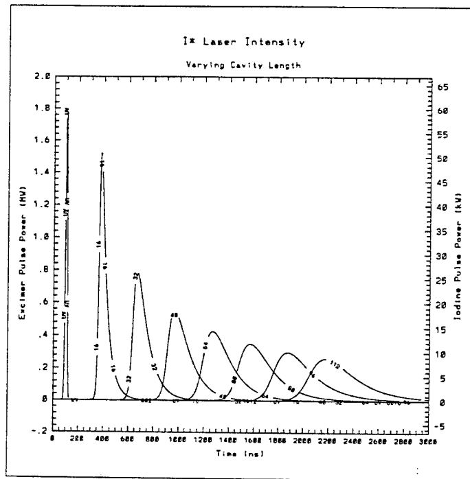
Figure 2-21a I* Laser Intensities for Various Cavity Lengths
