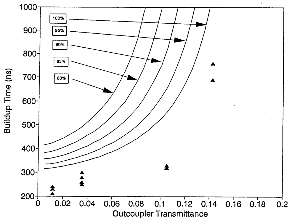
Figure 4-9 Error Bounds Due to Uncertainty of Quantum Yield
