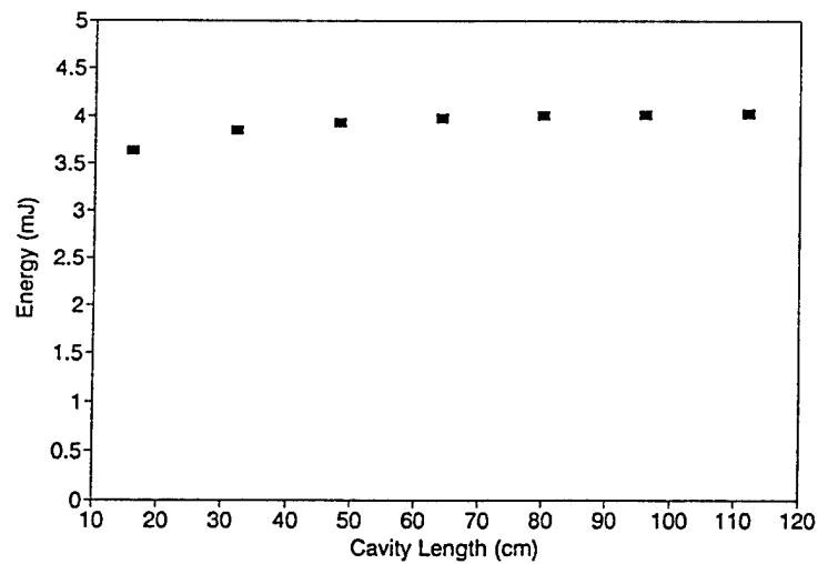
Figure 2-21b I* Laser Energy versus Cavity Length
