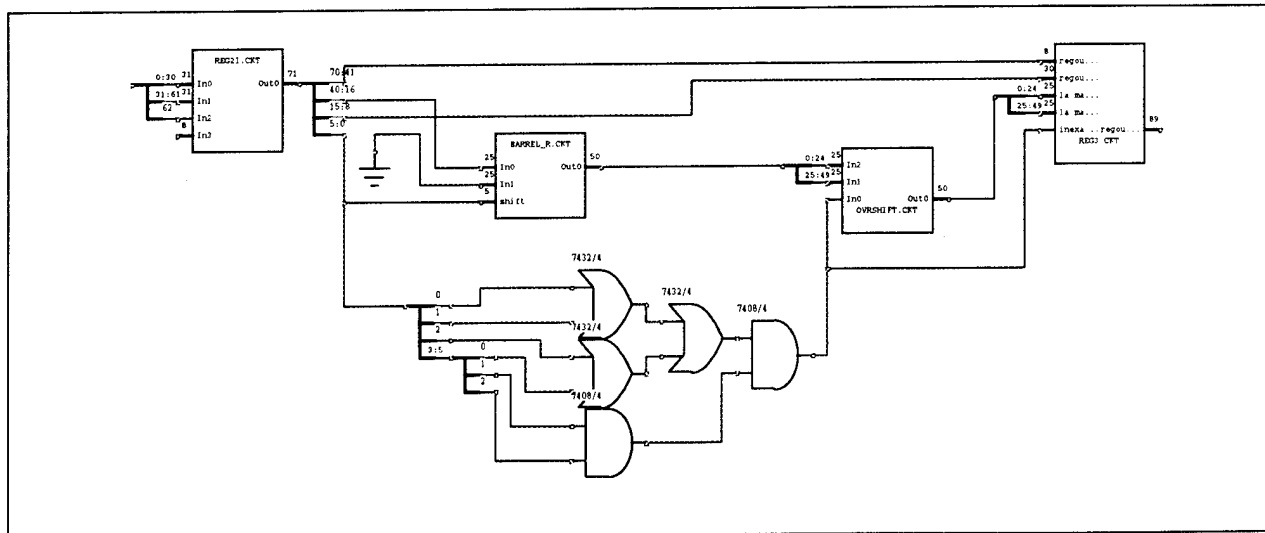
Figure 15 - Floating Point Adder Stage 4
