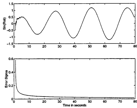
FIGURE 5.16 Sin \phi Estimate from Kalman Filter
