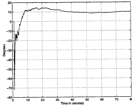
FIGURE 5.26 Slow Spinning Kalman Filter Roll Error with Y and Z axis Rate Gyro Bias Active and Noise with a Shell Roll Rate of 0Hz
