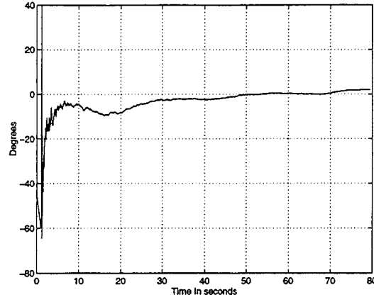
FIGURE 5.22 Roll Error Performance of Slow Spinning Kalman Filter with all Errors Active
