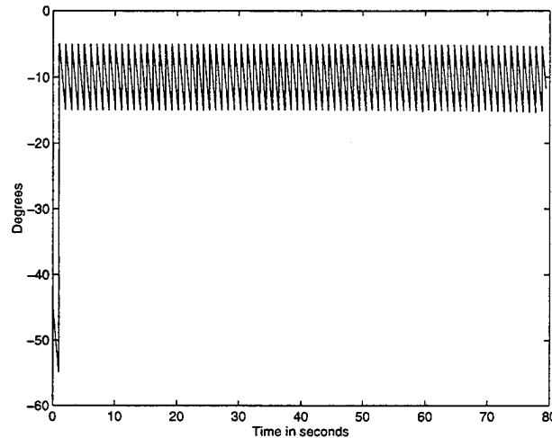
FIGURE 4.3 Slow Spin Rate Roll Error \Delta t = 1 sec
