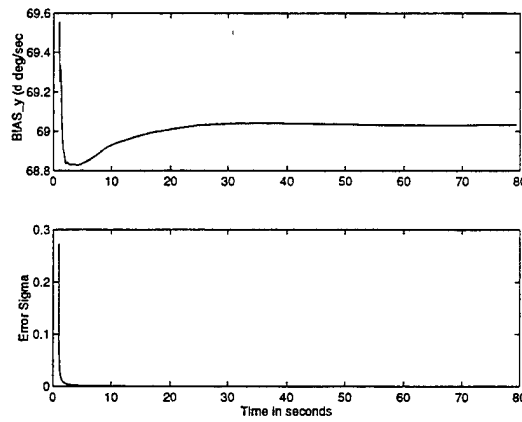
FIGURE 5.4 Y Body Axis Rate Gyro Bias Estimate from Kalman Filter
