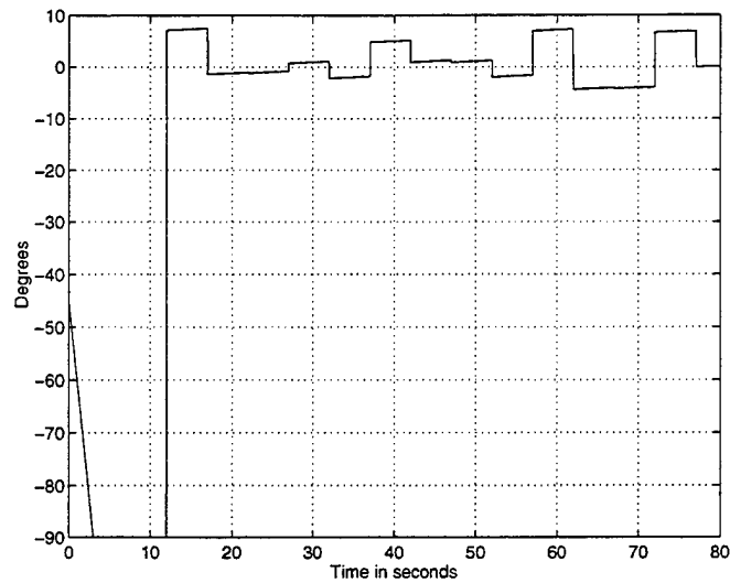
FIGURE 4.6 Final Slow Spin Algorithm Performance with Sensor Noise On, P=0.04167\text{Hz} , System Rate = 1000Hz
