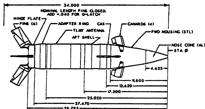
FIGURE 1.1 Guided Munition Round
