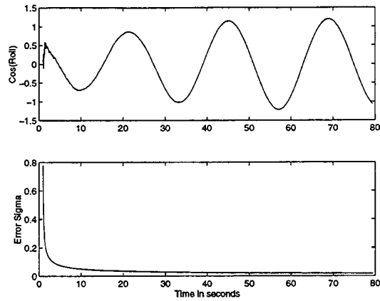
FIGURE 5.15 Cos \phi Estimate from Kalman Filter
