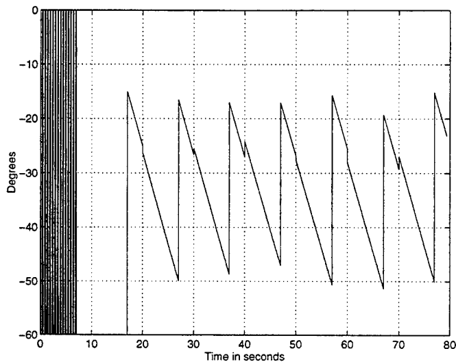
FIGURE 3.10 Roll Error with Non-Orthogonality of 0.096 rad in both X and Y Body Axis Rate Gyro in the X-Y Plane with Bias Error Correction Implemented
