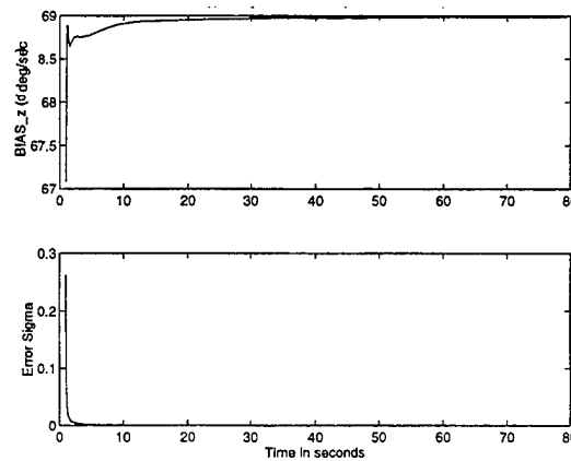
FIGURE 5.5 Z Body Axis Rate Gyro Bias Estimate from Kalman Filter
