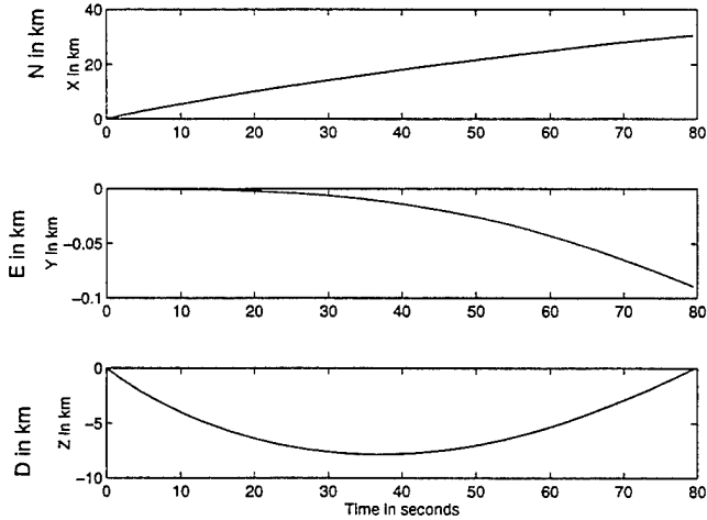
FIGURE 2.1 Non-Spinning Artillery Shell Position in NED
