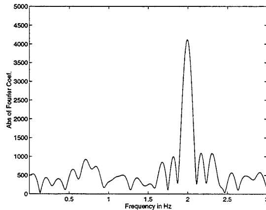
FIGURE 3.12 1,500,000 Point NFFT of 10s \text{Sin}\phi Data Sampled at 1000Hz
