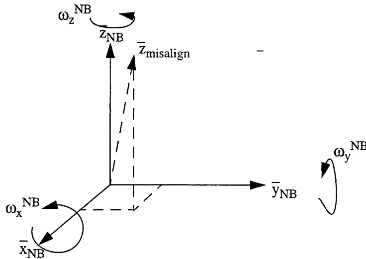
FIGURE 6.2 Non-Orthogonality Error Depiction
