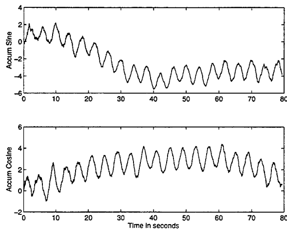
FIGURE C.1 Accumulated Sine and Cosine Roll from Algorithm
