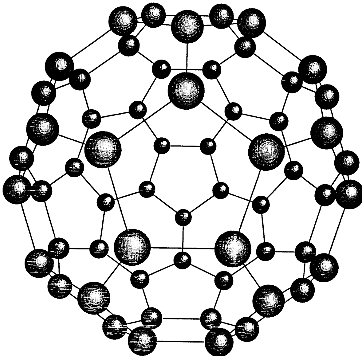
Figure 1. The structure of C_{60} .
