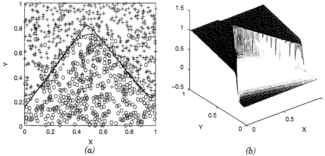
Figure 8. (a) A contour plot of the decision surface generated by the evolved cascaded network with two hidden units. The dashed line represents the optimal decision boundary. (b) The decision surface generated by the two hidden node CCLA.
