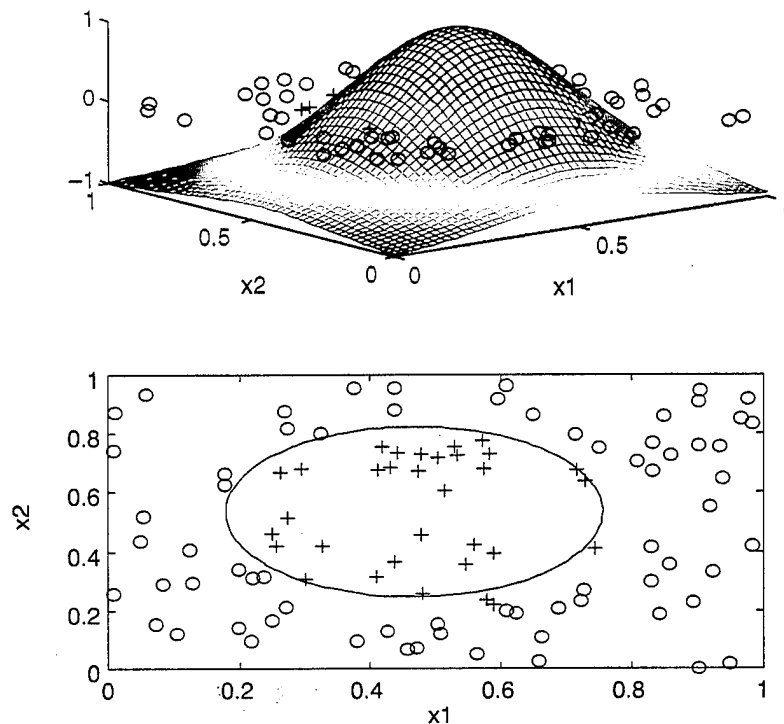
Figure 11. The mesh and contour plots of the decision surface generated by the mixture activation function for the clustered data set.
