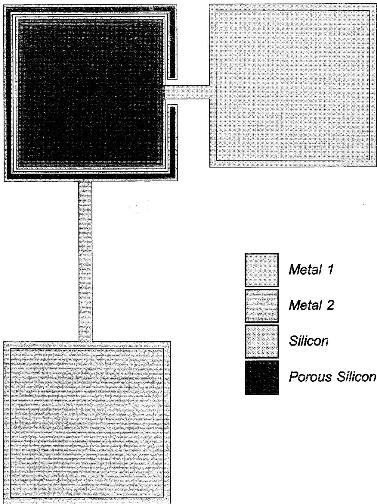
Figure 7. Porous SOS LED design.
