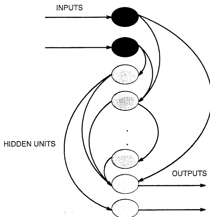
Figure 2. A general feedforward network.
