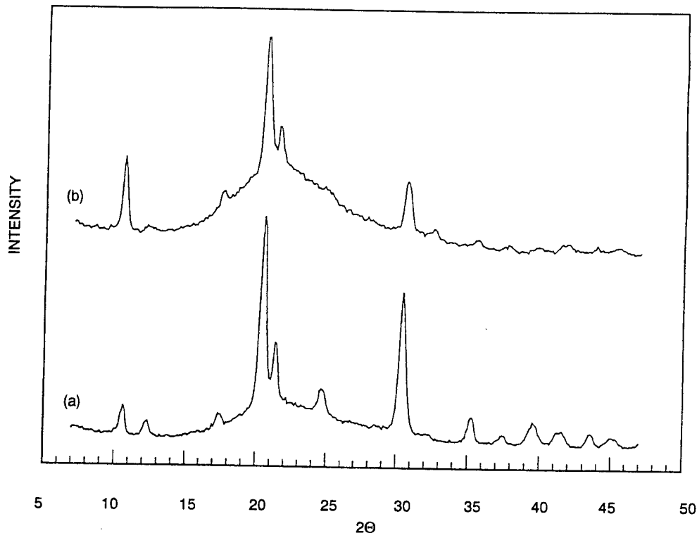
Figure 4. X-ray diffraction patterns for (a) the Rb_3C_{60} of figure 1b after an additional 2 days at 250°C under dynamic vacuum and (b) the K_3C_{60} after 6 days at 100°C under dynamic vacuum.
