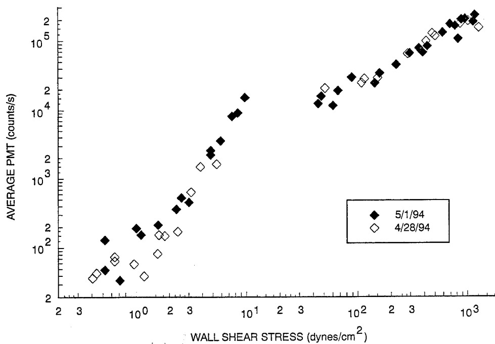
Figure 1. Representative San Diego Bay PMT levels as a function of wall shear stress.
