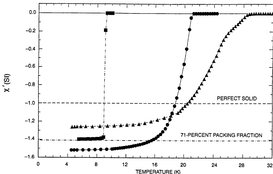
Figure 5. The real part of the AC volume susceptibility versus absolute temperature for a powdered sample of \text{Rb}_3\text{C}_{60} annealed as for the sample of figure 2a ( \blacktriangle ), a powdered sample of \text{K}_3\text{C}_{60} annealed as for the sample of figure 2b ( \bullet ), and a sample of 60 mesh niobium metal powder ( \blacksquare ).
