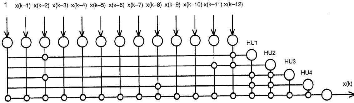
Figure 6. The resulting architecture for the CCLA-EP with complexity regularization. The solid circles represent active connections.
