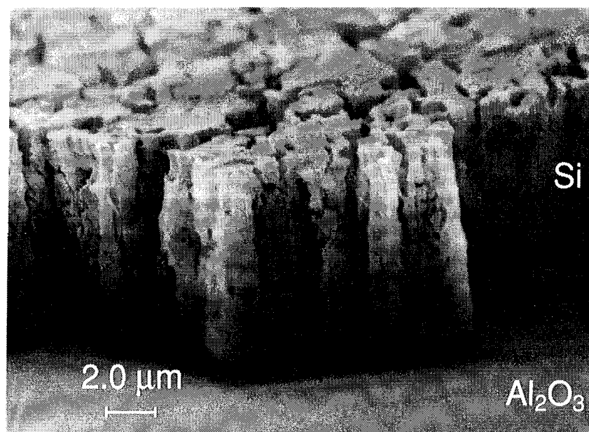
Figure 3. SEM cross section of porous SOS.
