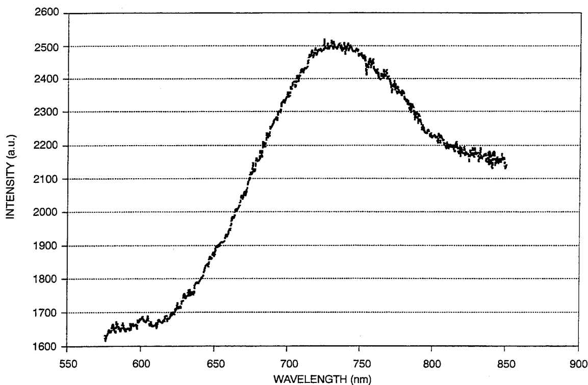
Figure 10. SOS microplasma LED emission spectrum.
