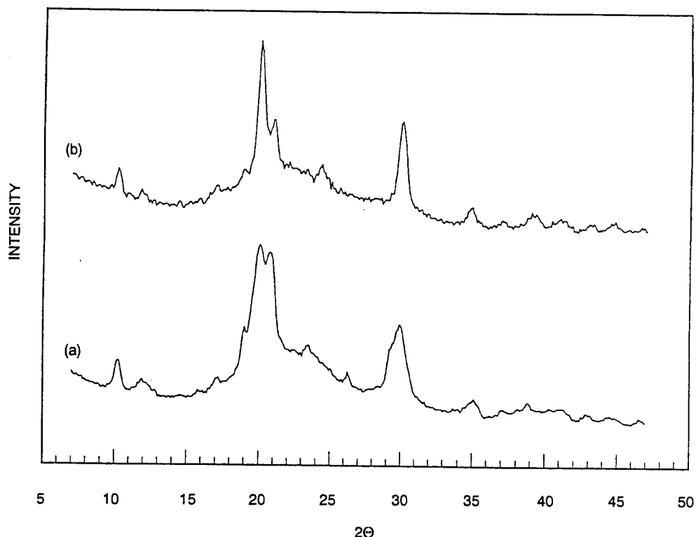
Figure 3. X-ray diffraction patterns for (a) the as made \text{Rb}_3\text{C}_{60} and (b) the \text{Rb}_3\text{C}_{60} after 3 days at 150°C under dynamic vacuum.
