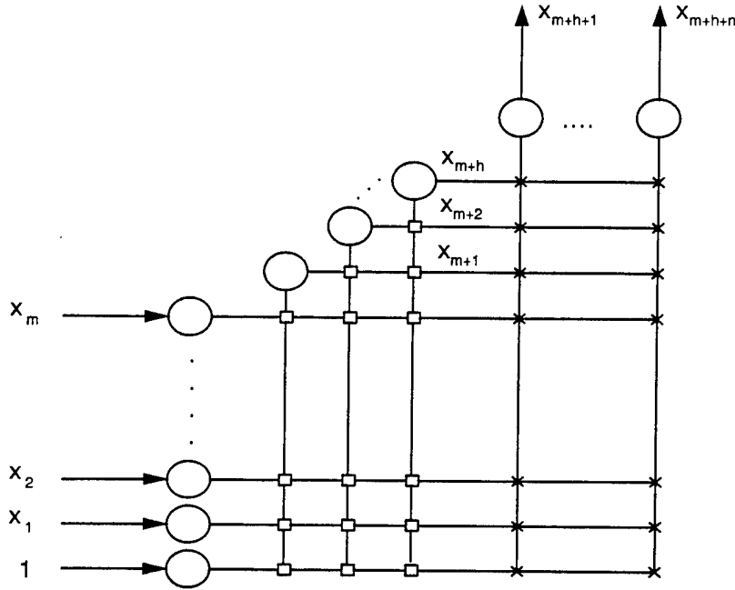
Figure 3. The cascade-correlation network structure. The boxes \square indicate weights that are frozen when the unit is incorporated into the network. The crosses \times indicate weights that are modified after a new hidden unit is incorporated.
