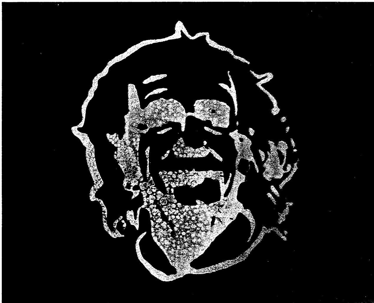
Figure 6. Photolithographically patterned porous silicon.
