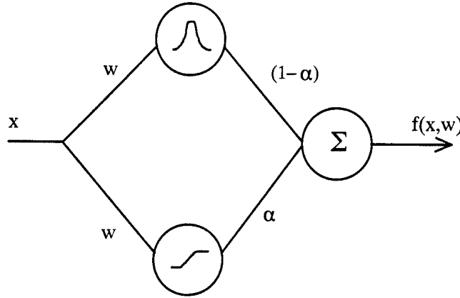
Figure 9. The mixture activation function model employs a combination of kernel and ridge-type functions.
