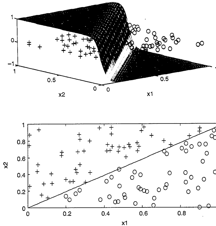
Figure 10. The mesh and contour plots of the decision surface generated by the mixture activation function for the linearly separable data set.
