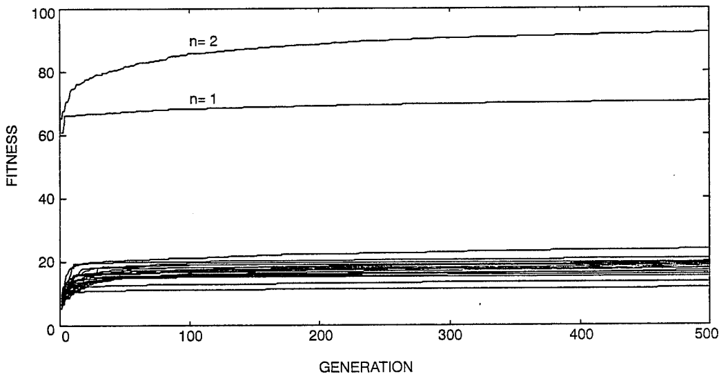
Figure 7. The correlation of the best candidate node in the population. The highest correlations correspond to the first ( n = 1 ) and second ( n = 2 ) hidden units.
