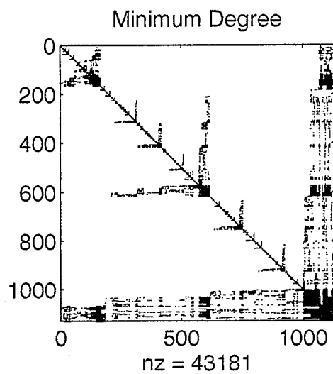
Figure 4. Sparsity structure of R^T + R for problem pilot.
