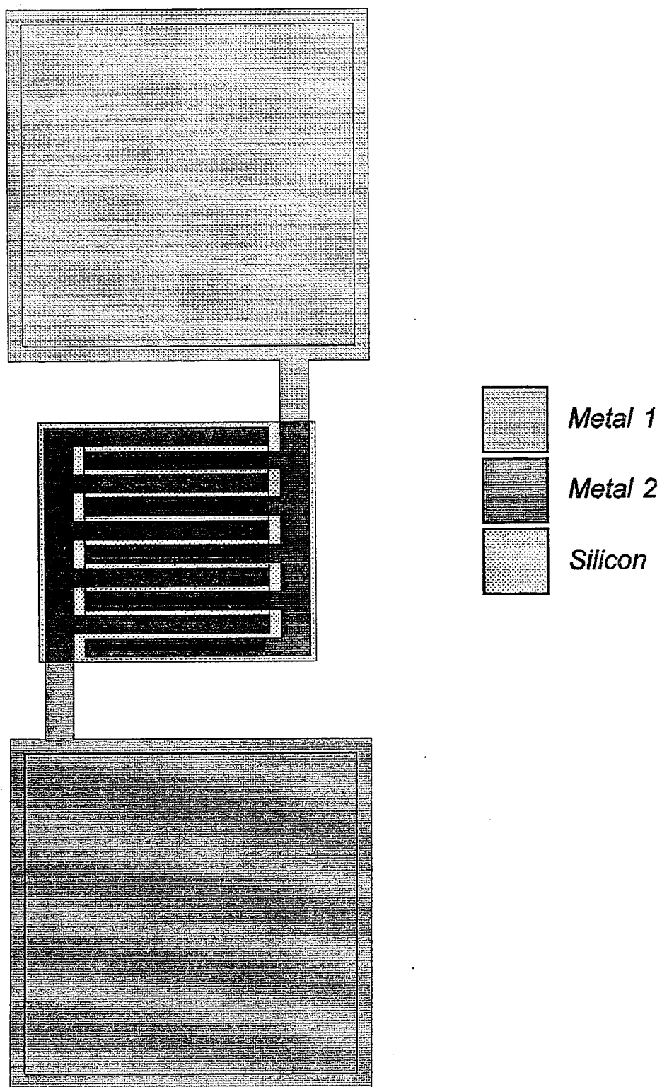
Figure 11. Ultrathin SOS microplasma LED design.
