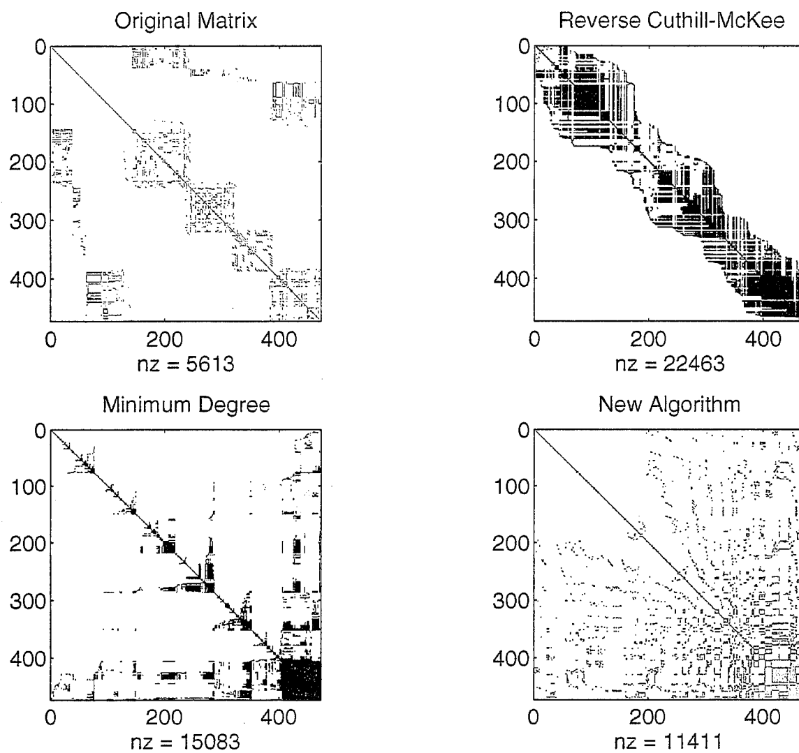
Figure 2. Sparsity structure of R^T + R for problem scfxm1 .
