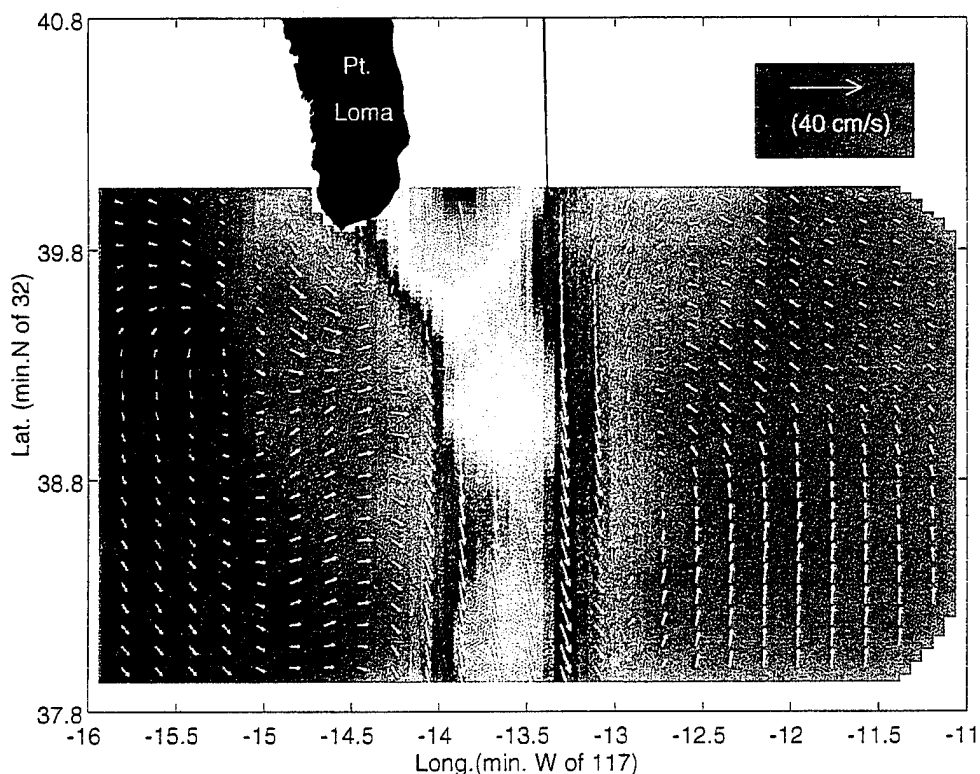
Figure 1. Flow and tracer fields off the mouth of San Diego Bay showing the structure of the outflow jet and the large-scale eddy structure associated with the tidal pumping mechanism.
