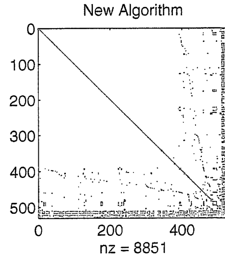
Figure 3. Sparsity structure of R^T + R for problem seba .
