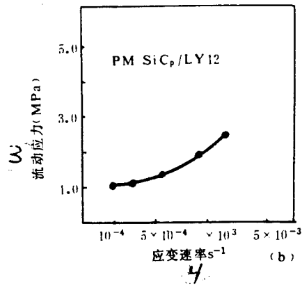
Fig.1 Influences of Strain Rate on Flow Stress
