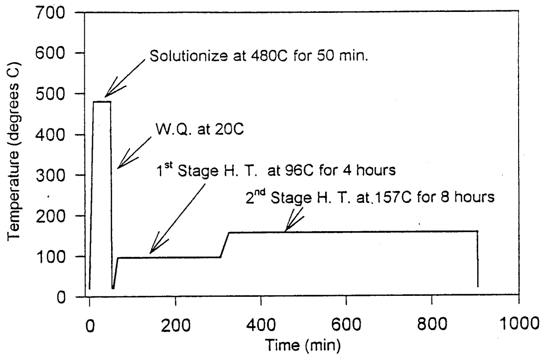
Figure 2.7 Typical two-stage heat treatment to achieve a -T6 temper in an Al 7075 alloy.
