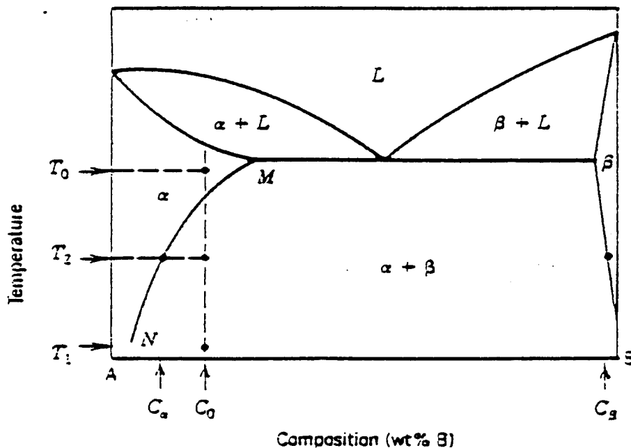
Figure 2.8 Hypothetical phase diagram for a precipitation hardenable alloy of composition C_0 . From Ref. [7].
