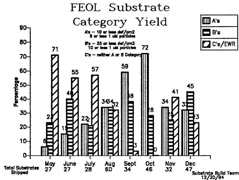
Figure 17. Substrate Fabrication Yield by Product Category. Category A has < 10 defects/cm 2 and < 5 defects larger than 1.0μm in size. Category B has < 25 defects/cm 2 and < 10 defects larger than 1.0μm in size. Category C has > 25 defects/cm 2 or > 10 defects larger than 1.0μm in size.
