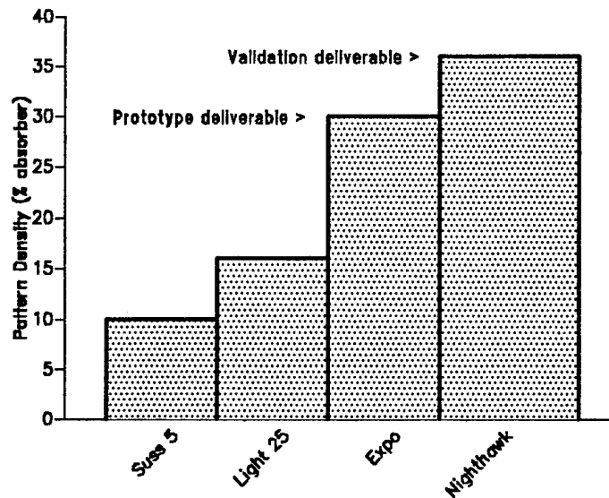
Figure 16. Pattern Density Increase
