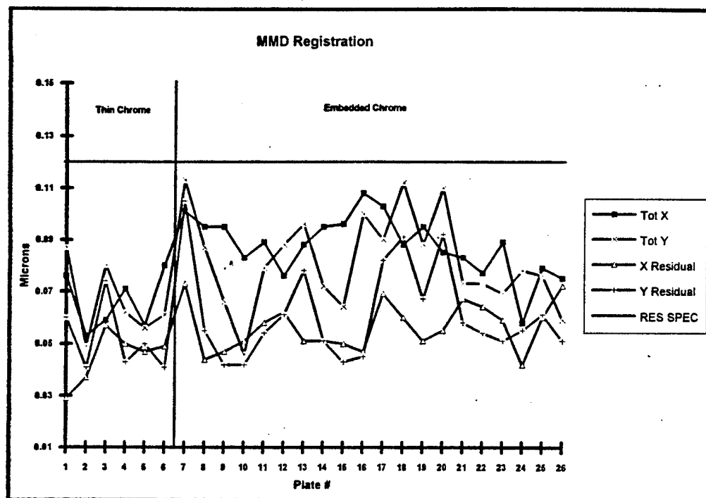
Figure 25. MMD Registration
