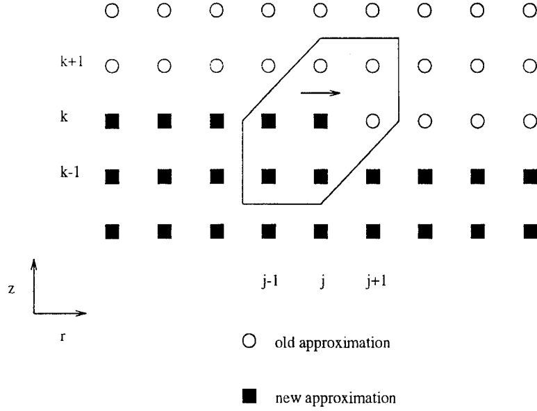
Figure 8. Gauss-Seidel sweep.
