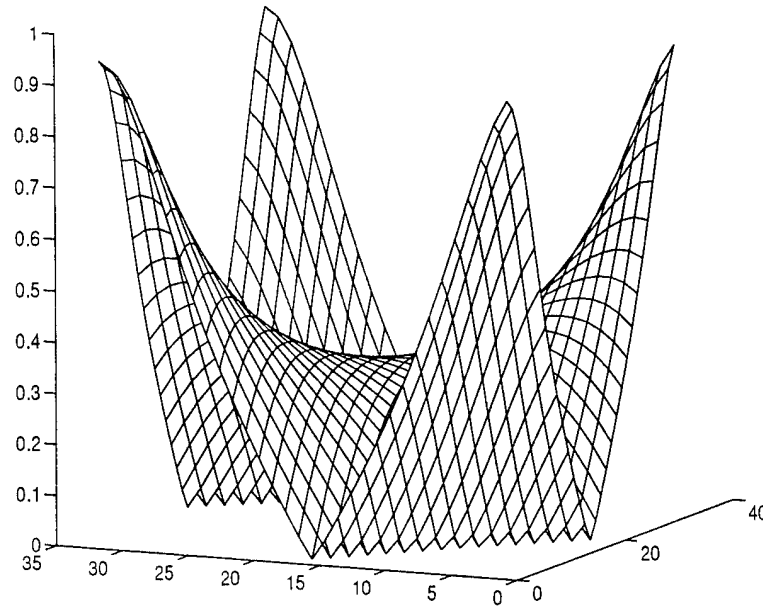
Figure 15. Ratio of amplitudes of new to old Fourier coefficients, Gauss-Seidel relaxation: N = 32 , \alpha = 1 , j = N - 1 . Frequency ranges are as in Figure 11.
