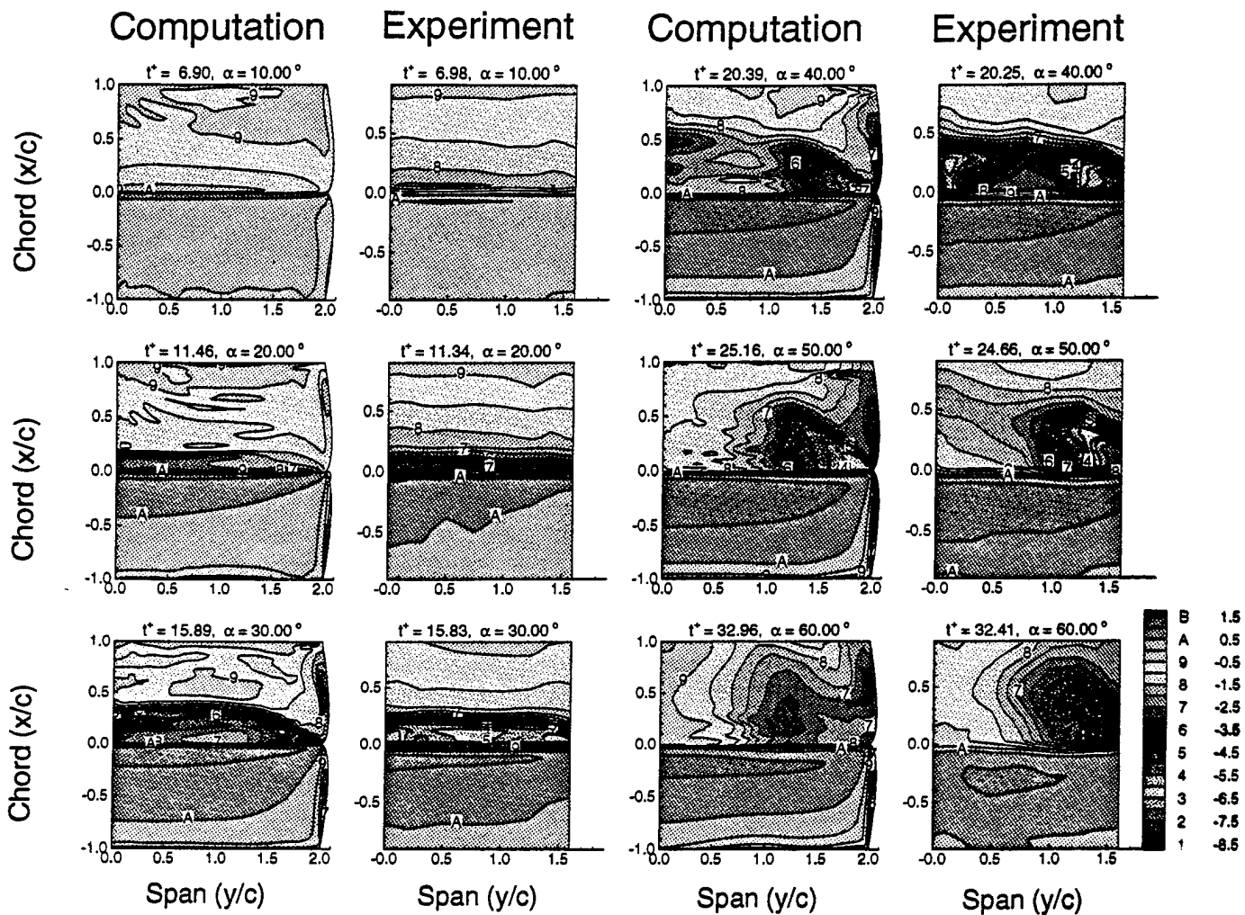
Fig. 11 Comparison of computational and experimental pressure coefficients \Omega^+ = 0.2 , Re_\infty = 56000
