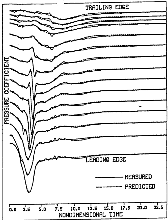
Fig. 2. Unsteady surface pressures for constant rate pitching, nondimensional pitch rate 0.20.
