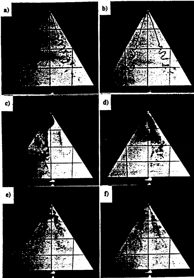
Fig. 3 Photographs of delta wing vortices where a) and b) show burst delay at 20 deg with increased V_j , c) and d) show oscillation of burst vortices at 30 deg, and e) and f) show stabilization and delay of burst as V_j increases: a) \alpha = 20 deg, V_j = 0.0 ; b) \alpha = 20 deg, V_j = 8.0 ; c) \alpha = 30 deg, V_j = 0.0 , time 1; d) \alpha = 30 deg, V_j = 0.0 , time 2; e) \alpha = 30 deg, V_j = 5.0 ; and f) \alpha = 30 deg, V_j = 8.0 .
