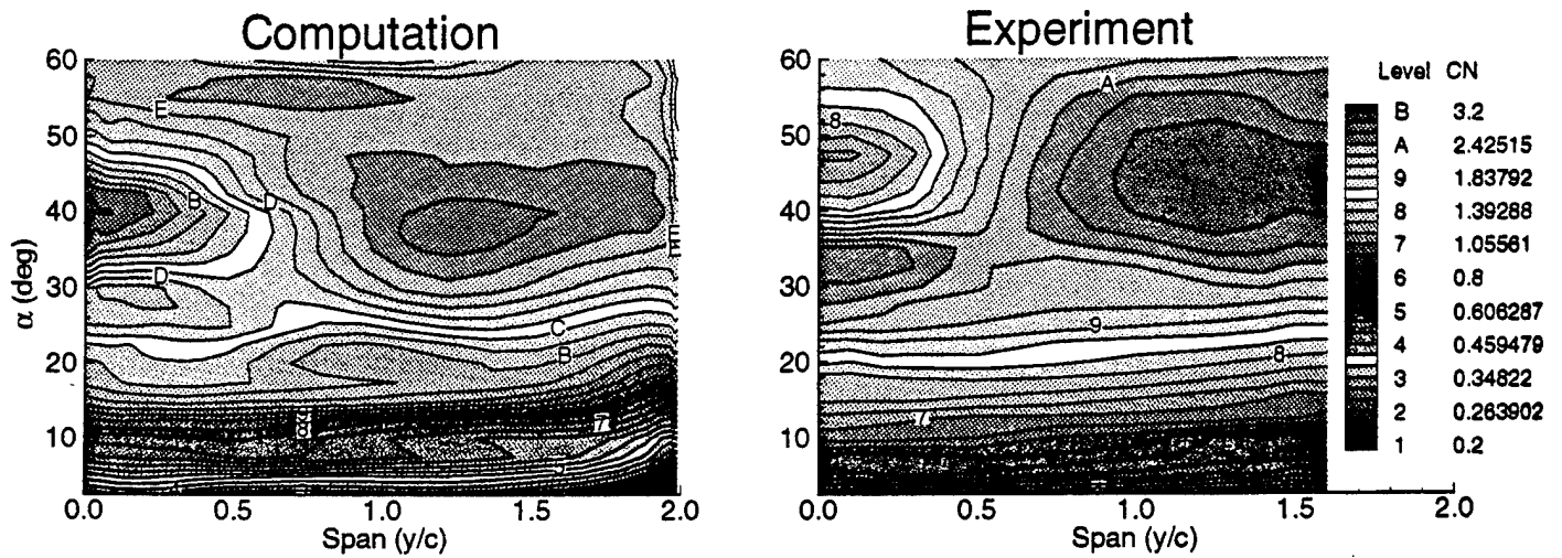
Fig. 16 Comparison of computational and experimental normal force coefficients \dot{\Omega}^+ = 0.1 , Re_m = 56000
