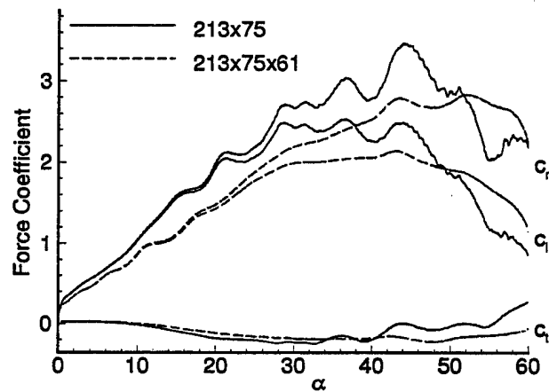
Fig. 14 Comparison of normal and tangential force coefficients for 3D finite wing and equivalent 2D airfoil, \Omega^+ = 0.2 , Re_\infty = 56000
