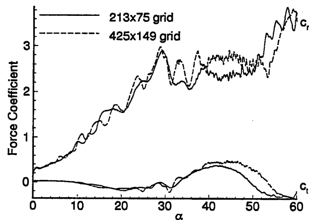
Fig. 17 Spatial accuracy for equivalent 2D airfoil, \dot{\Omega}^+ = 0.1 , Re_m = 56000 Grid Sizes: 213x75 425x149
