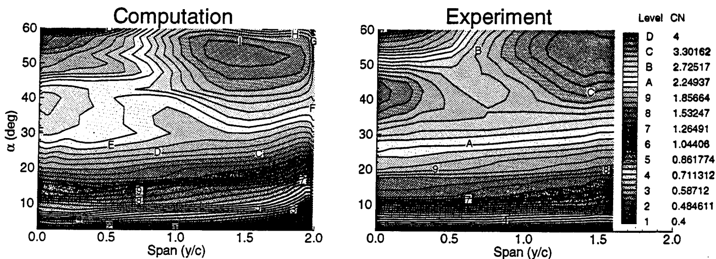
Fig. 12 Comparison of computational and experimental normal force coefficients \Omega^+ = 0.2 , Re_\infty = 56000
