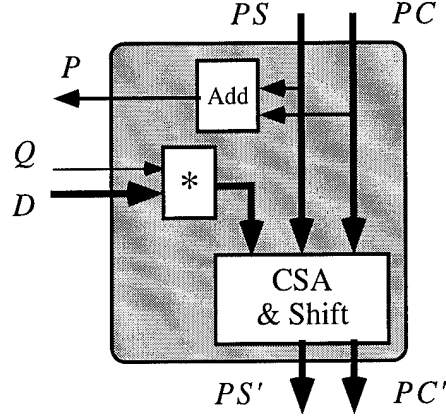
Figure 3: Divider stage modified for generation of PD table
