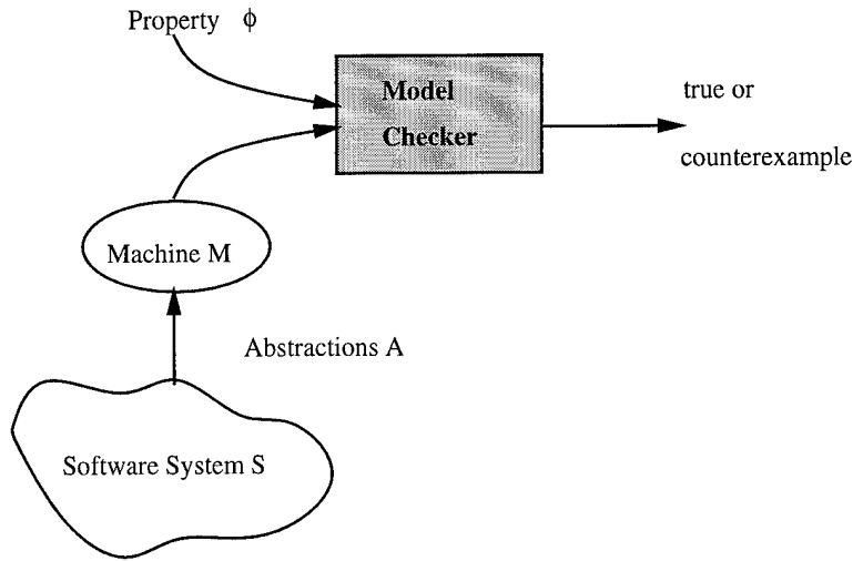
Figure 1: Model Checking Software
