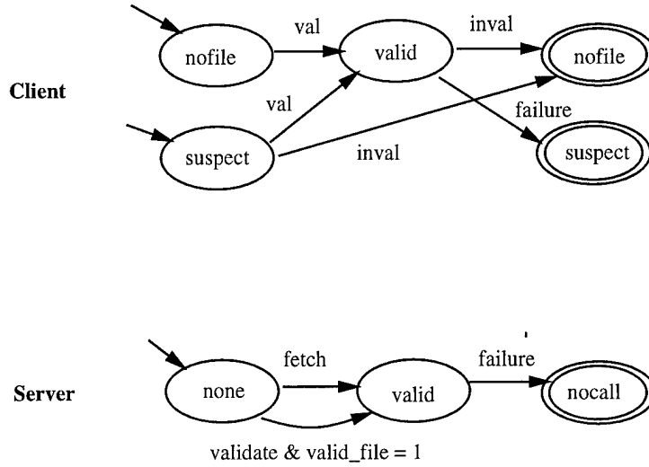
Figure 5: State Transition Graphs for AFS-2
