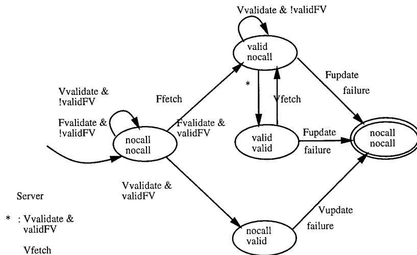
Figure 9: State Transition Diagrams for Coda
