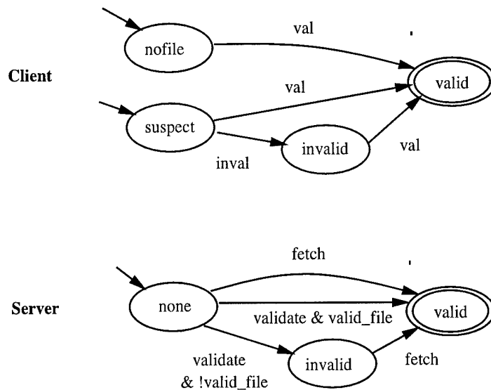
Figure 2: State Transition Graphs for AFS-1
