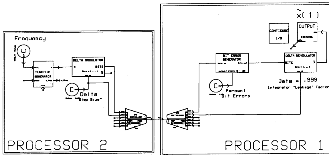
Figure 5.6: Delta Modulation example
