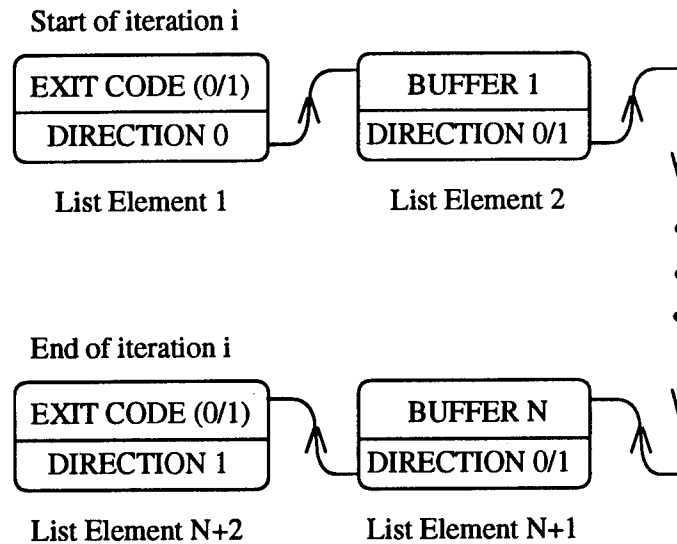
Figure 5.4: Linked List & Operation of DMA
