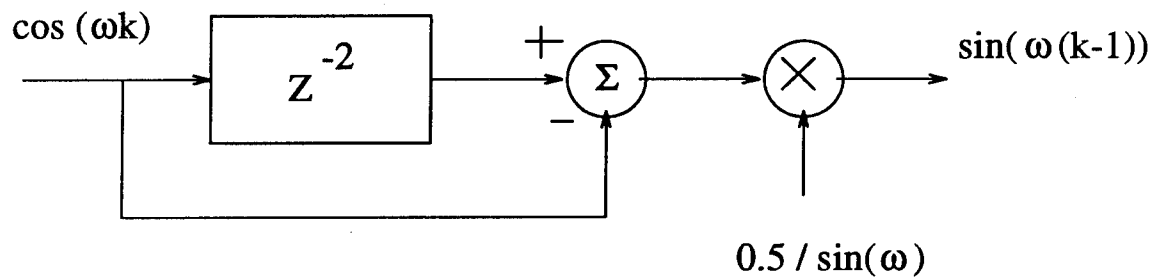
Figure 4.2: Derivative Block Implementation
