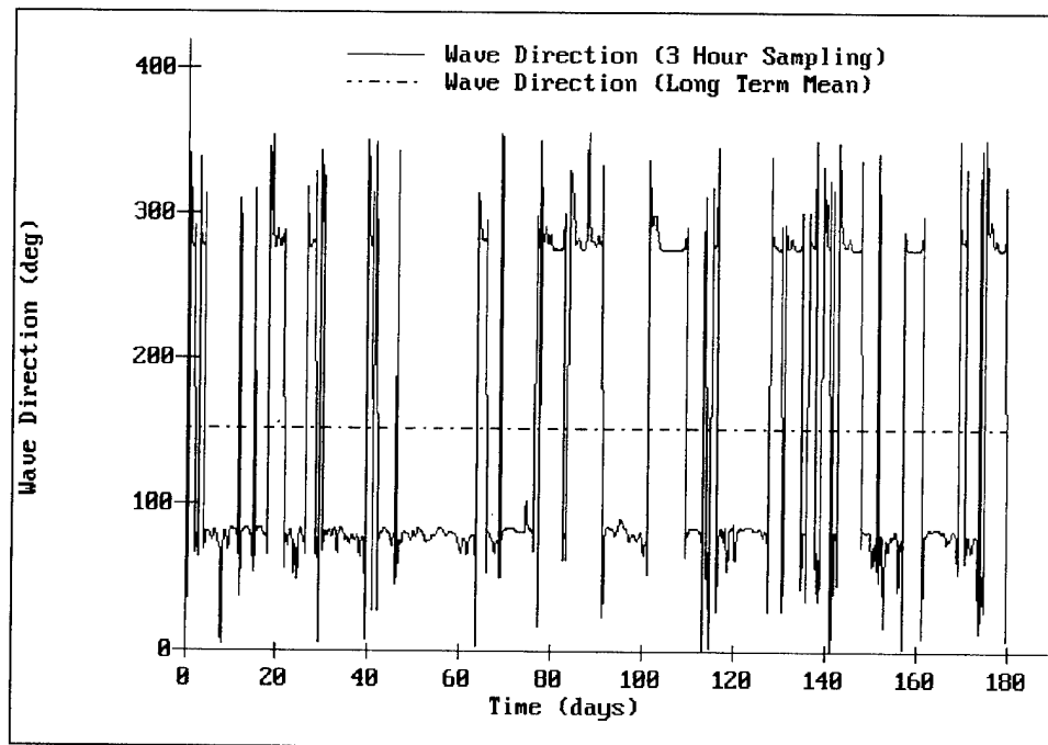
Figure 20. Wave direction time series plot
