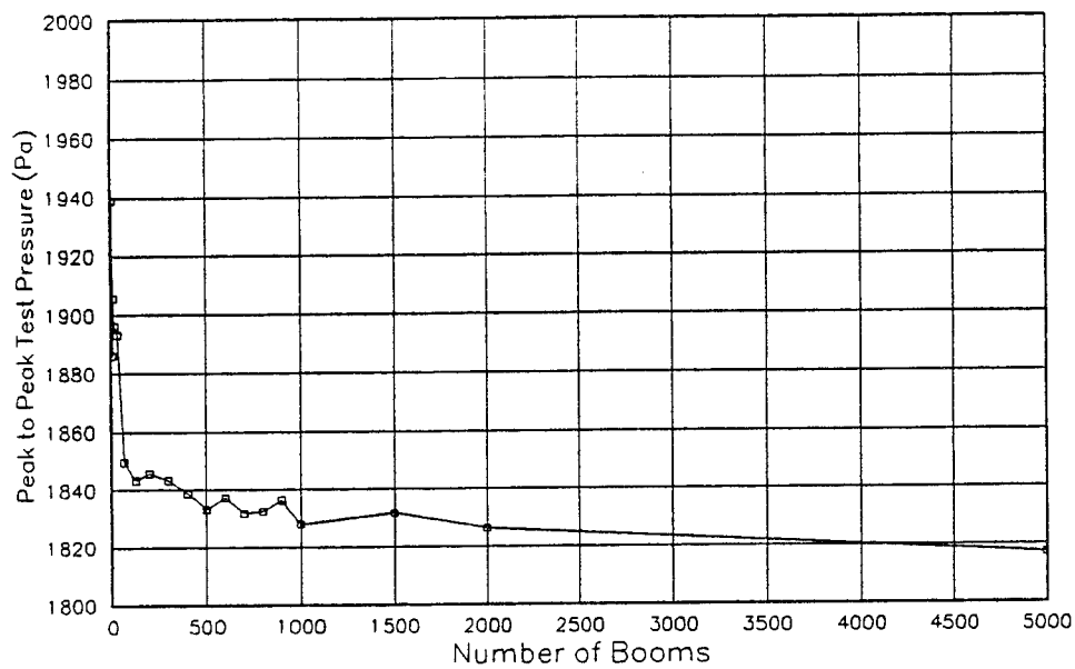
Figure A-1. Peak to Peak Test Pressure vs Boom Number (Strong Plaster, 20 psf)
