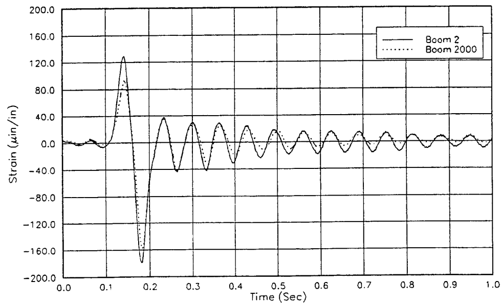
Figure A-38. Strain (Uniaxial 1) vs Time for Boom 2 and 2000 (Strong Plaster, 20 psf )
