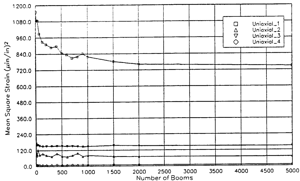
Figure A-37. Mean Square Strain vs Boom Number (Strong Plaster, 20 psf)
