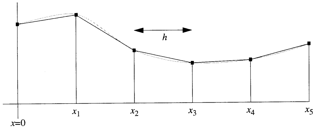
Figure 5.1. Example of trapezoidal integration.
