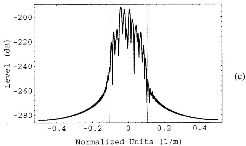
Figure 5.3. DFT's of: a) modeled field, b) Green's function, c) product.
