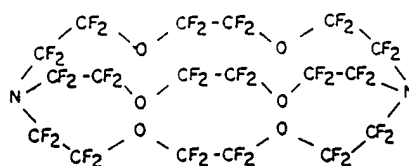
Figure 9. The perfluorocryptand[2.2.2].
