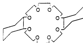
dicyclohexano-24-crown-8 ether
