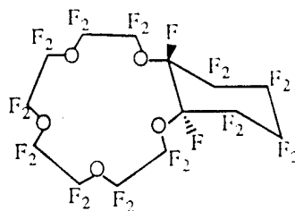
perfluoro- trans -cyclohexano-15-crown-5 ether
