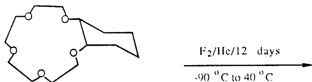
cyclohexano-15-crown-5 ether trans - and cis - isomers
