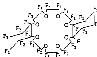
perfluorodicyclohexano-24-crown-8 ether
