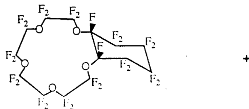
perfluoro- cis -cyclohexano-15-crown-5 ether
