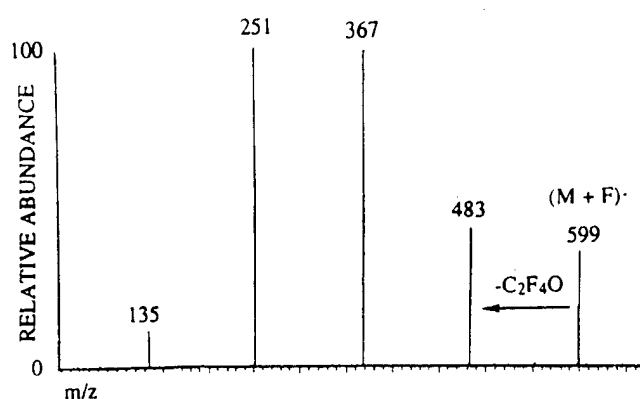
Figure 13. Collisionally activated dissociation mass spectra of the (M + F)^- ion of perfluoro [15]crown-5 acquired with a triple quadrupole mass spectrometer.
