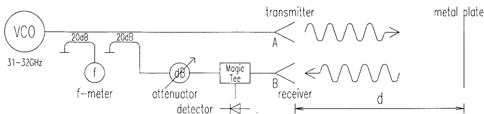
Fig. 1 Circuit diagram
