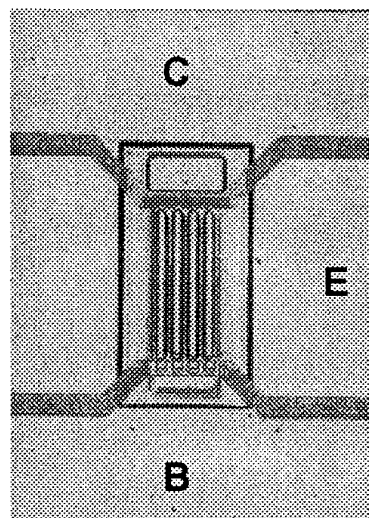
Figure 5: Photograph of a 4-emitter fingers HBT
