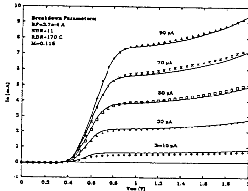
Fig.1 InP/InGaAs HBT Measured and Modeled ICE-VCE Characteristics
