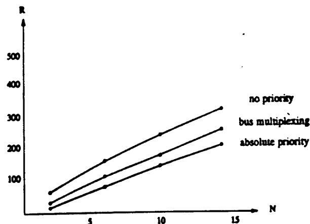
Figure 3. Response time vs. number of stations for 8K bits packets
