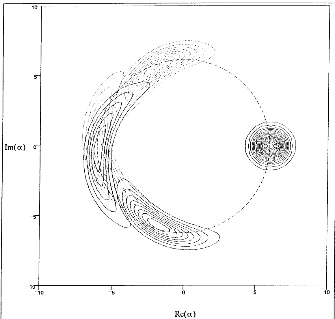
Figure 26. Q distribution for the plus (solid lines) and minus (dotted lines) branches for \bar{n}=36 , \varepsilon=0.3 at \omega t=0, 300 , and 500 . As the branches overlap, the revival occurs. The dashed line indicates \alpha=6=\sqrt{\bar{n}} .
