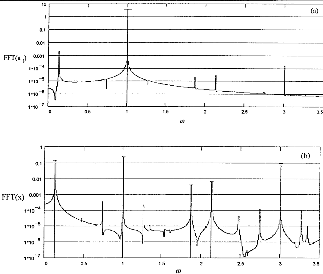
Figure 8. FFT of \alpha_1(t) (a) and x(t) (b) for \varepsilon=1.0 , \bar{n}=1024 , \gamma=-0.1 \pi . In addition, vertical bars indicate magnitude and location of peaks predicted by the Autler-Townes model (Eq. 2.9).
