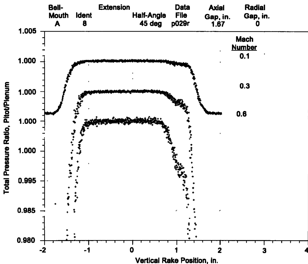
Figure 35. Effect of Mach number variation on total pressure profiles in Bellmouth A for large axial gap and zero radial gap.
