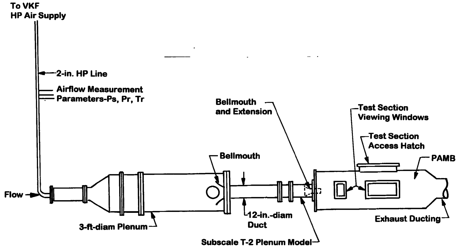
Figure 2. Schematic of Icing Research Cell R1D.
