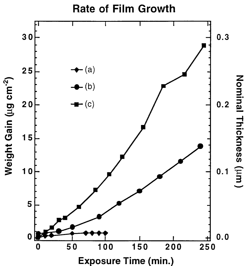
Figure 1. Weight gain on an Al film measured by a quartz crystal microbalance. (a): Weight gain due to water condensation. (b): Weight gain during \text{H}_2\text{SO}_4 exposure. \text{P} = 0.036 Torr, 80% relative humidity. (c): Weight gain for \text{P} = 0.18 Torr, 30% relative humidity.
