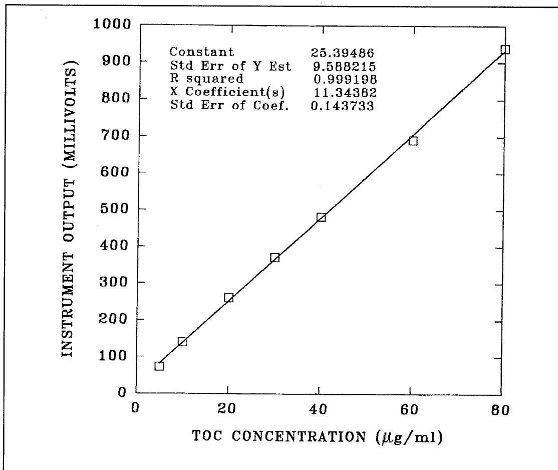
Figure 1. Total organic carbon standard calibration curve
