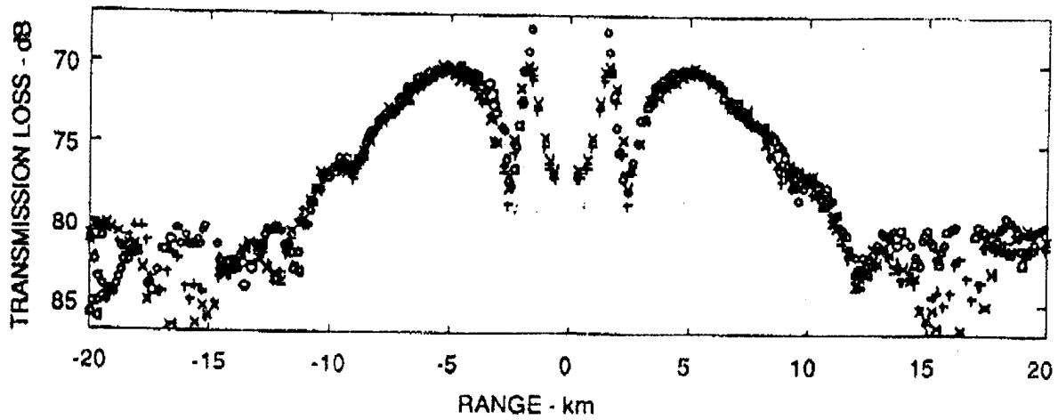
(a) 10 Hz PEAK ARRIVALS FROM THE SURFACE
