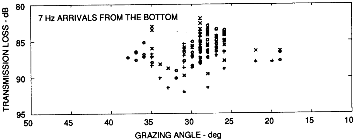
(a) TRANSMISSION LOSS versus ANGLE IN THE RANGE INTERVAL 35.3-44.6 km
