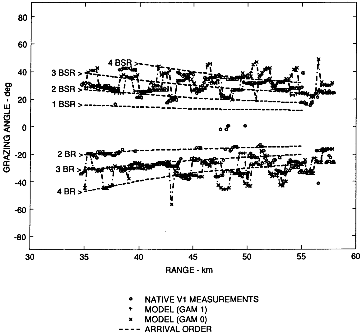
FIGURE 7.6 MEASURED AND MODELED (GAM 0 AND GAM 1 SEDIMENT MODELS) GRAZING ANGLES OF 7 Hz PEAK ARRIVALS FROM THE SURFACE AND FROM THE BOTTOM AT LONG RANGES
