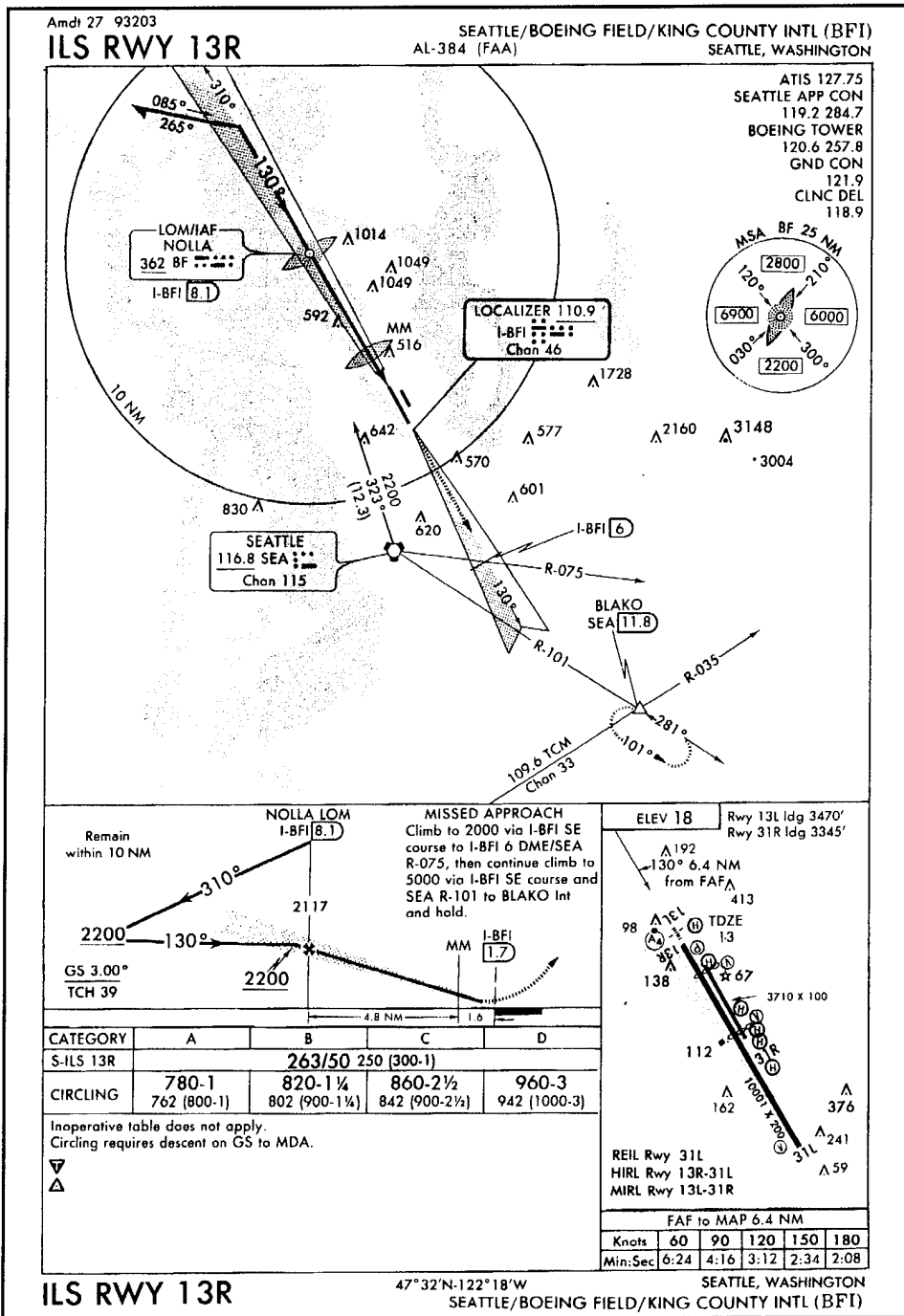
Figure 1-1. - Current Paper IAP Chart (See Section 5.1 for a complete description of current paper charts)
