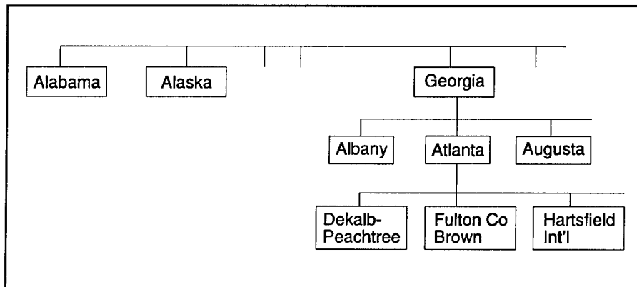
Figure 4-3. Hierarchical Menus
