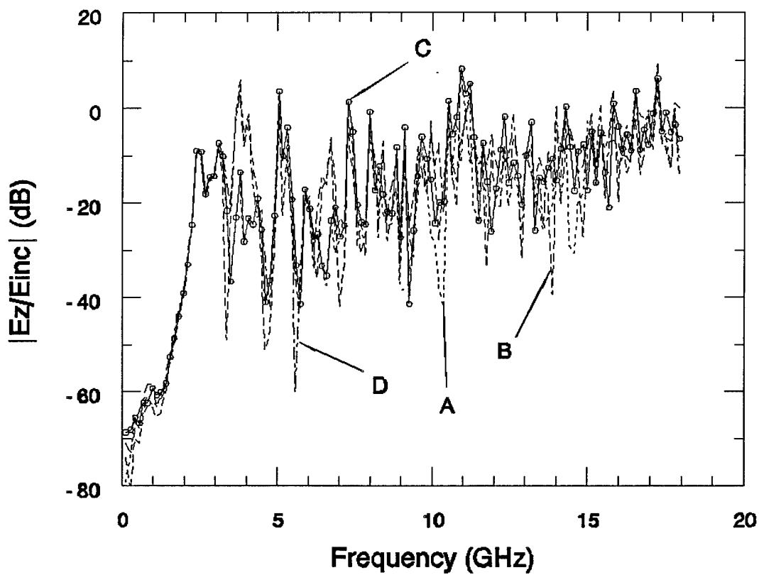
Fig 5 - Penetration of EM Fields into a Box with a Gasketed Lid [24].
