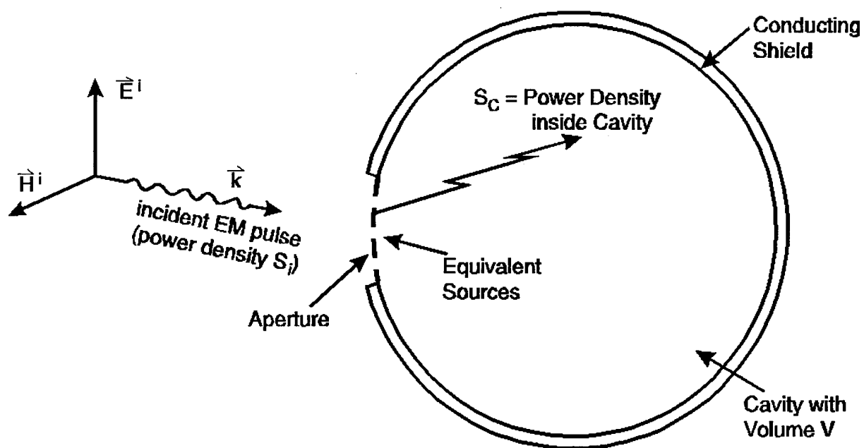
Figure 4 - Excitation of a Cavity with an Aperture
