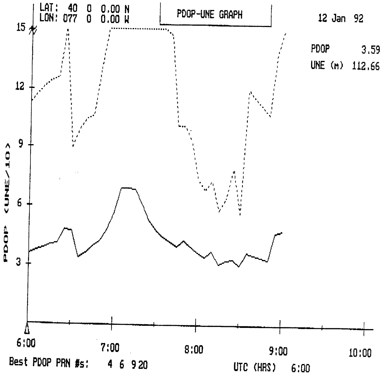
Figure B-8. PDOP At Mid-Latitudes. Mask Angle of 30 Degrees.
