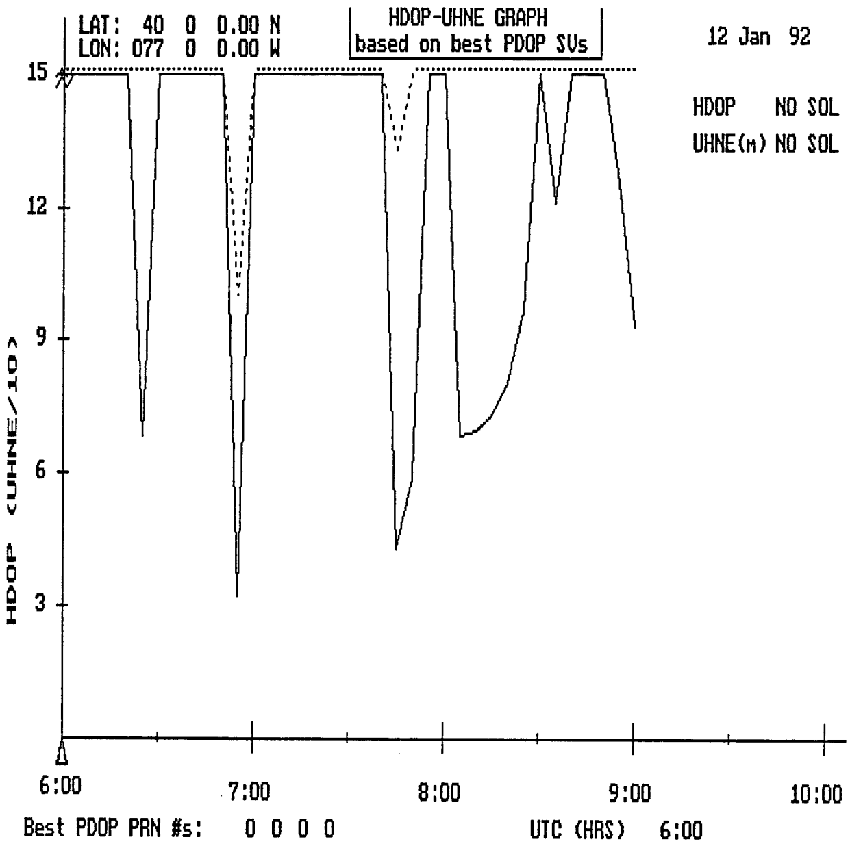
Figure B-12. HDOP At Mid-Latitudes. Mask Angle of 60 Degrees.(NO SOLUTION FOR PDOP)
