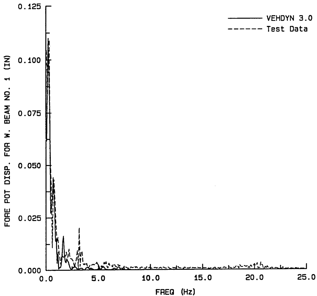
Figure A-49. Relative displacement frequency plot (frequency scale = 5.0 Hz/inch) of the forward-most axle with respect to the frame for a fully loaded HEMTT traveling at 1.82 miles per hour encountering a 1.00-inch-high obstacle.
