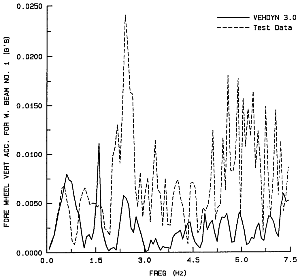
Figure A-67. Vertical acceleration frequency plot (frequency scale = 1.5 Hz/inch) of the forward-most axle for a fully loaded HEMTT traveling at 1.81 miles per hour encountering a 3.00-inch-high obstacle.
