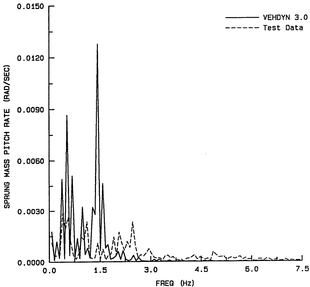
Figure A-117. Sprung mass pitch rate frequency plot for an empty HEMTT traveling at 1.80 miles per hour encountering a 3.00-inch-high obstacle.
