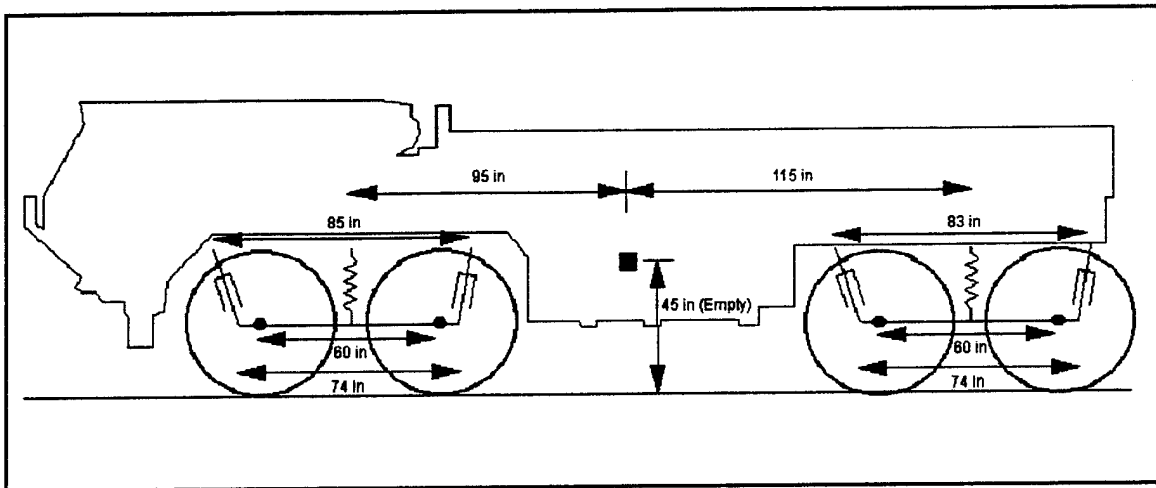
Figure 2-2. VEHDYN 3.0 Model of M977 HEMTT.
