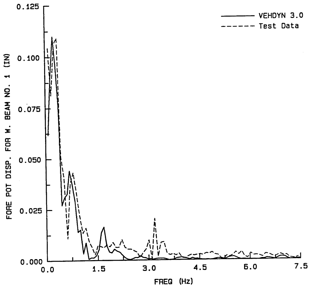
Figure A-48. Relative displacement frequency plot (frequency scale = 1.5 Hz/inch) of the forward-most axle with respect to the frame for a fully loaded HEMTT traveling at 1.82 miles per hour encountering a 1.00-inch-high obstacle.
