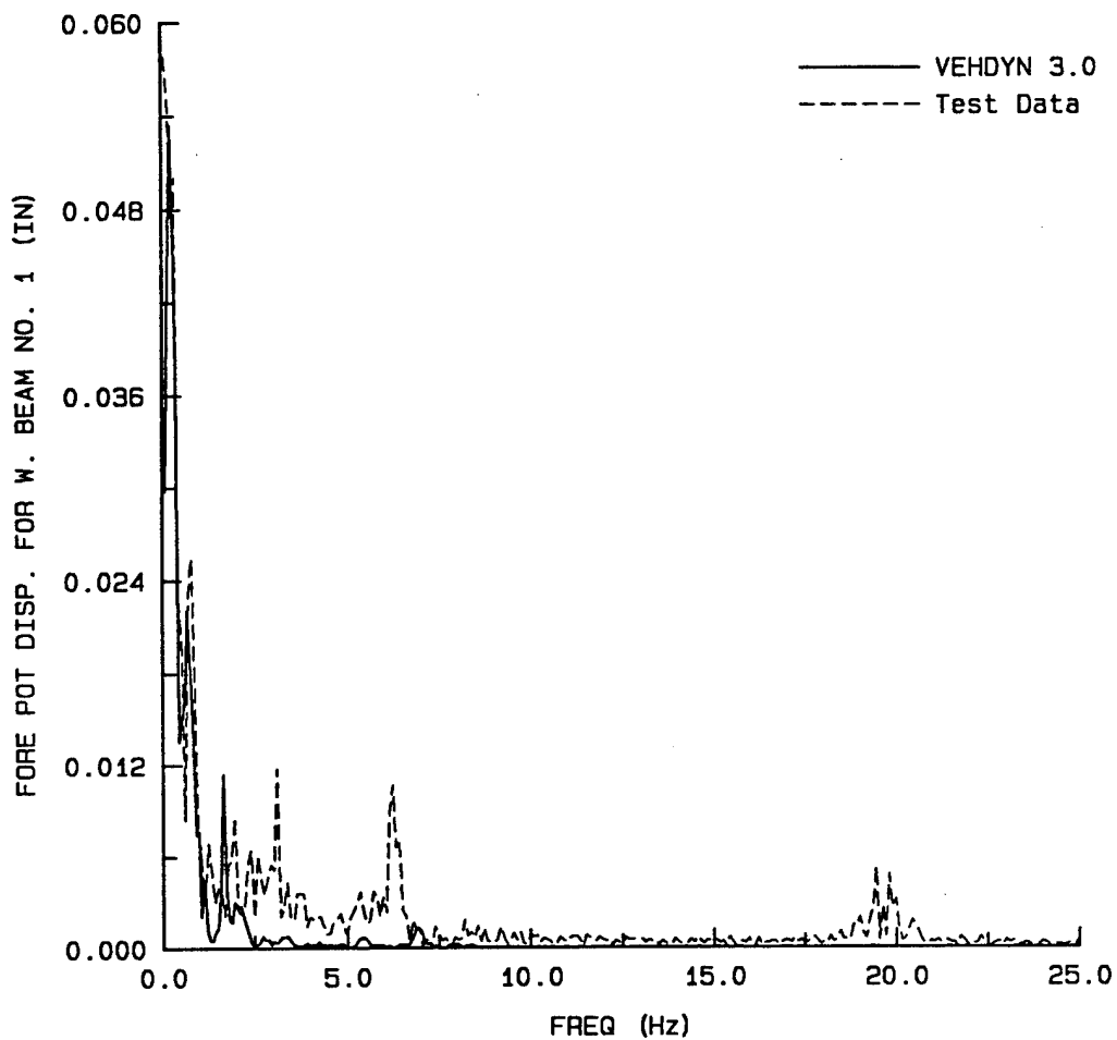
Figure A-38. Relative displacement frequency plot (frequency scale = 5.0 Hz/inch) of the forward-most axle with respect to the frame for a fully loaded HEMTT traveling at 1.80 miles per hour encountering a 0.50-inch-high obstacle.
