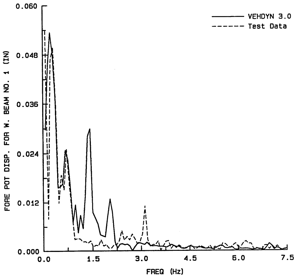
Figure A-92. Relative displacement frequency plot (frequency scale = 1.5 Hz/inch) of the forward-most axle with respect to the frame for an empty HEMTT traveling at 1.80 miles per hour encountering a 0.50-inch-high obstacle.
