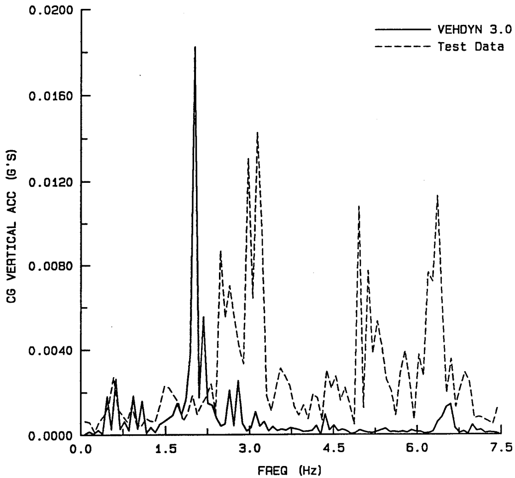
Figure A-97. CG vertical acceleration frequency plot (frequency scale = 1.5 Hz/inch) for an empty HEMTT traveling at 1.85 miles per hour encountering a 1.00-inch-high obstacle.
