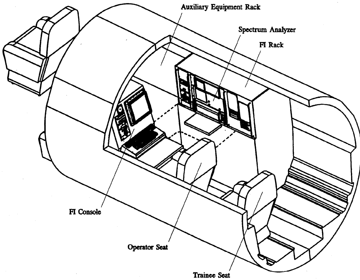
FIGURE 11 Accepted Workstation Layout
