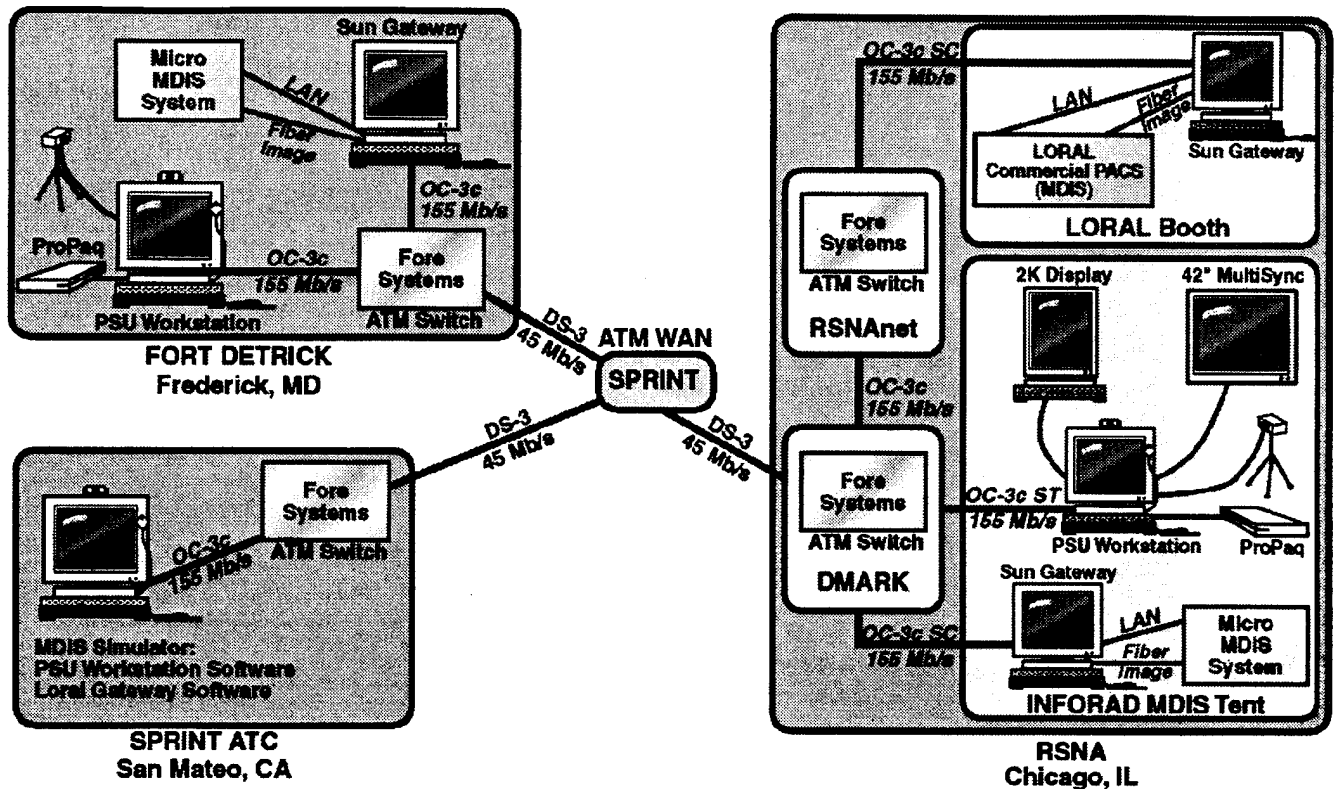
Figure 1. ATM WAN Testbed
