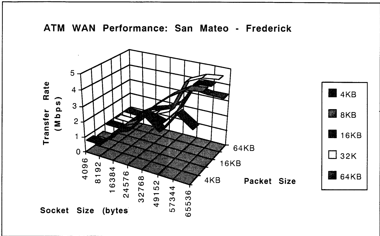
Figure 5. Socket to Socket Transfer Rates TCP/IP-ATM: WAN
