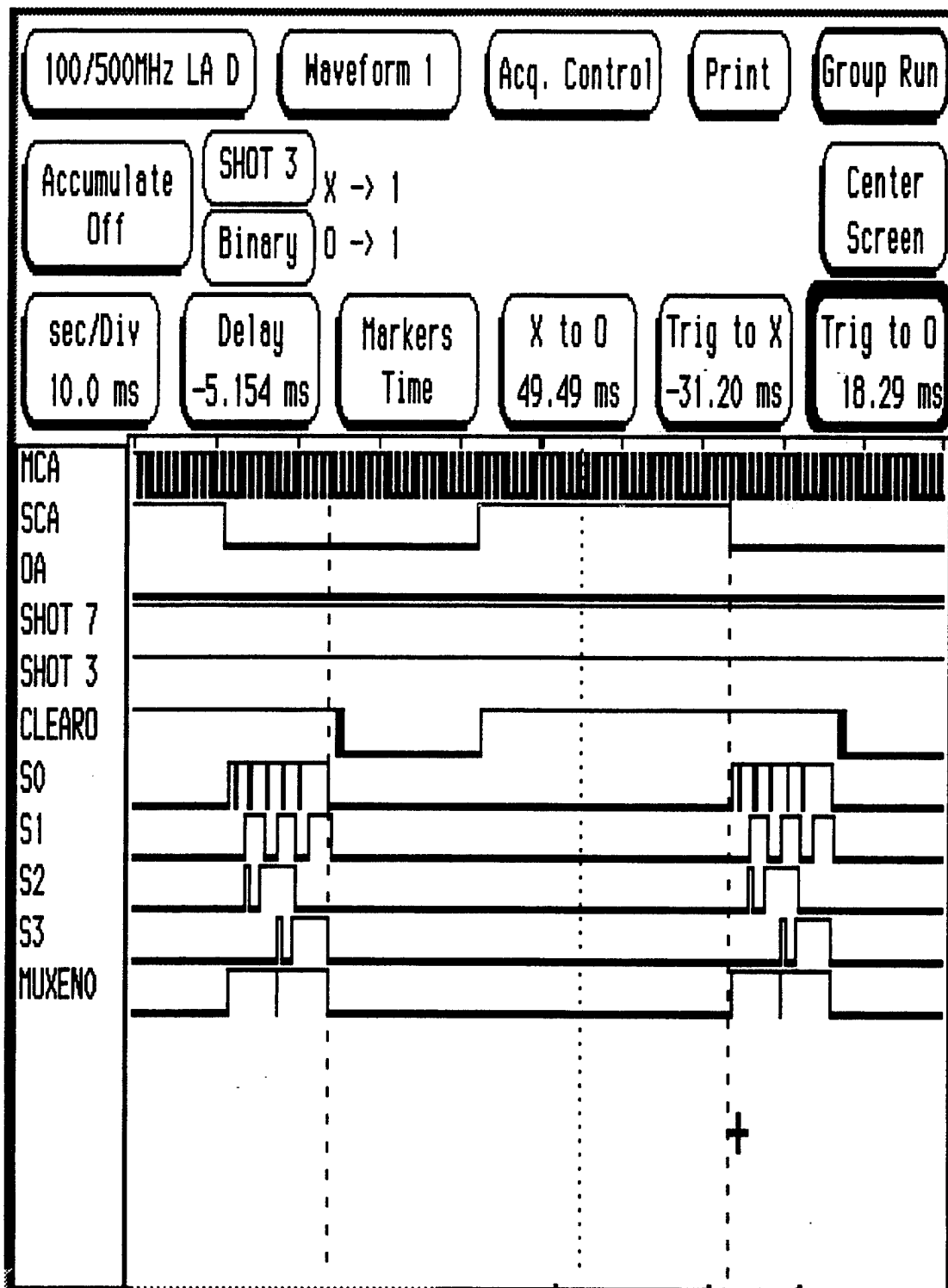
Figure 21. Chip 12 Waveforms
