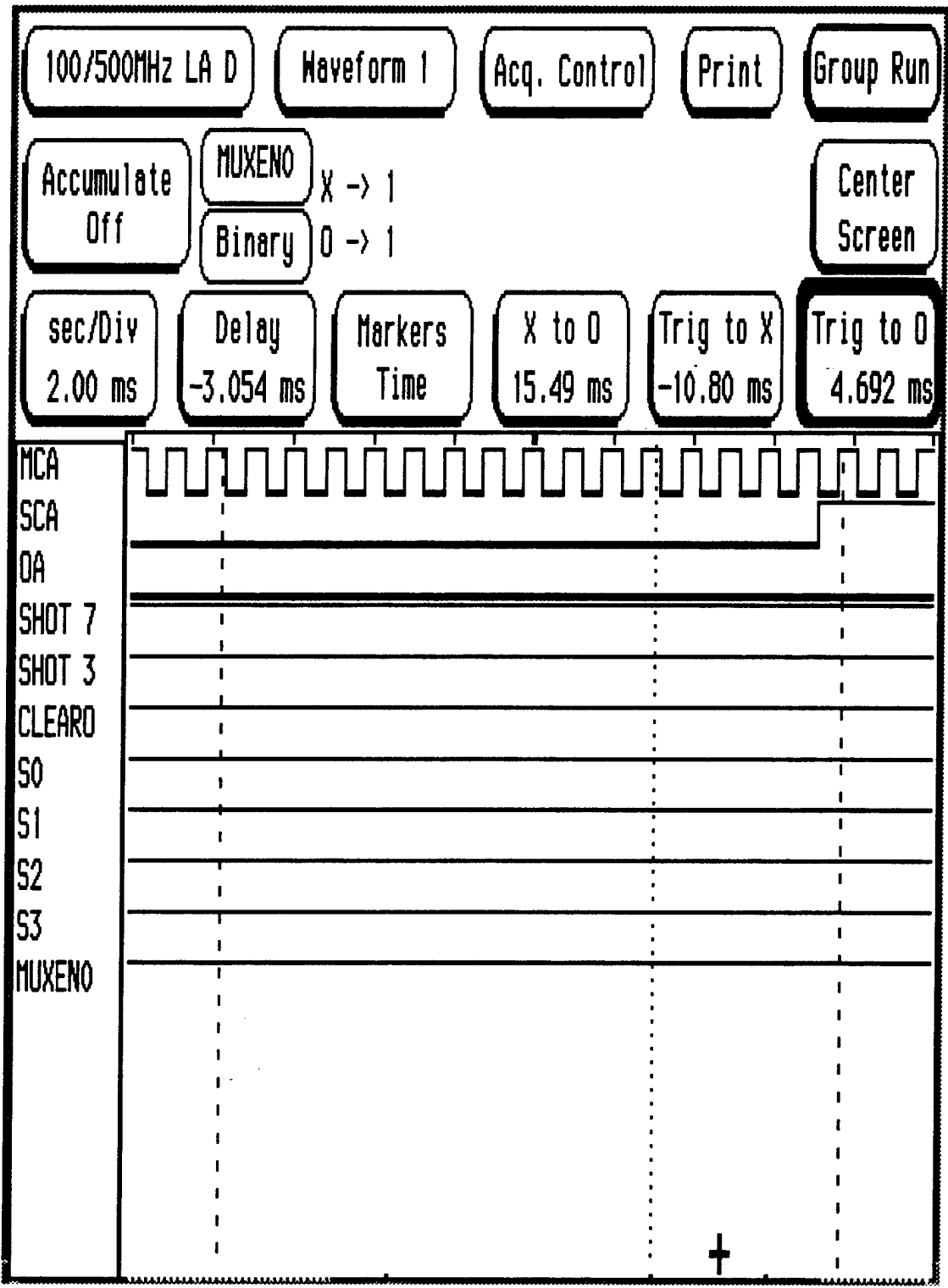
Figure 18. Chip 7 Waveforms
