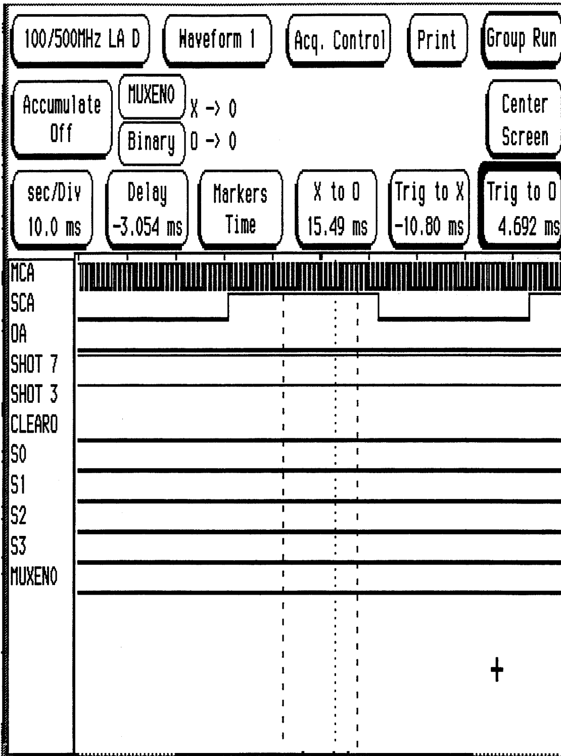
Figure 9. Chip 10 Waveforms
